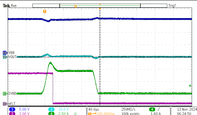
Figure 6-15. Switch Turn-Off
