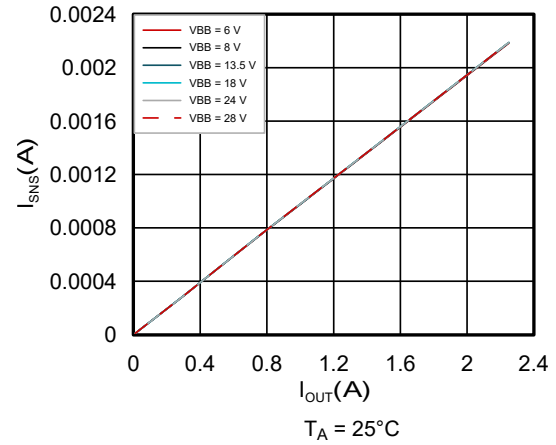
Figure 6-2. I_{SNS} vs I_{OUT} Over V_{BB} Voltage
