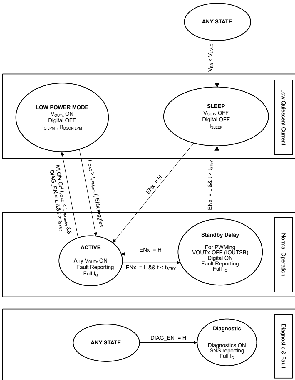
Figure 7-26. State Diagram
