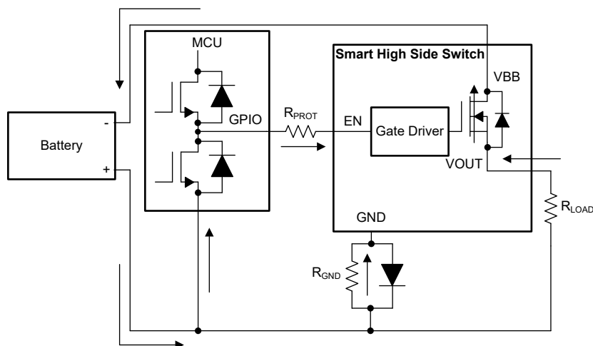
Figure 7-18. Reverse Battery Circuit
