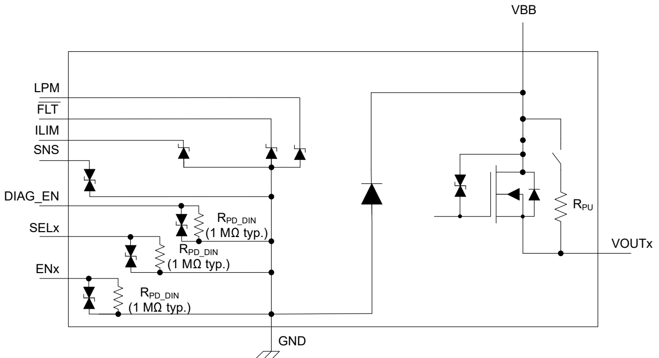
Figure 7-2. Internal Diodes Diagram
