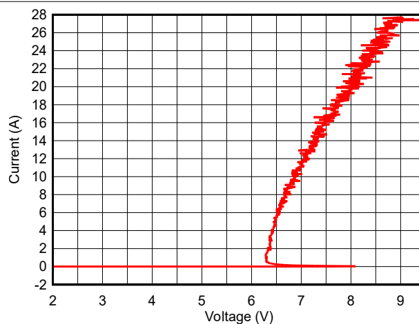
Figure 5-10. Positive TLP Curve (DPY)
