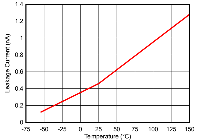
Figure 5-16. Temperature vs. Leakage Current (DPY)
