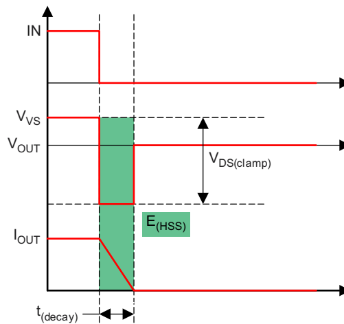
Figure 7-13. Inductive Load Switching-Off Diagram
