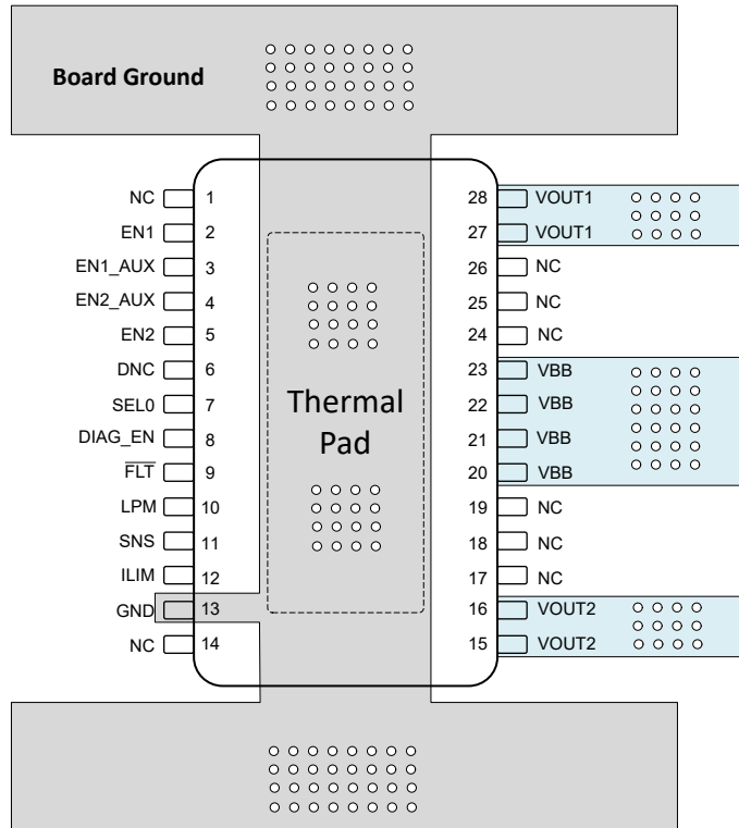
Figure 8-5. Layout Example Without a GND Network
