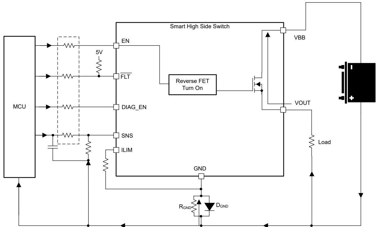
Figure 7-22. MCU I/O Protections
