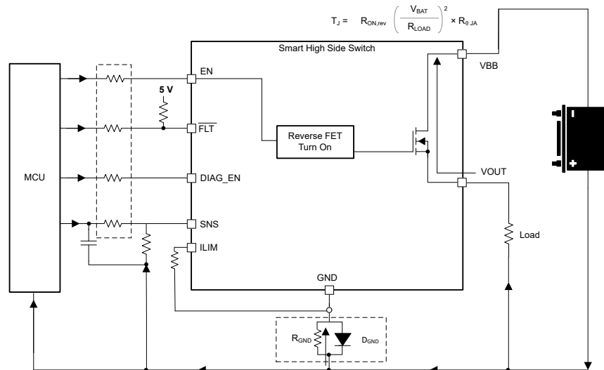
Figure 7-21. Reverse Protection With GND Network
