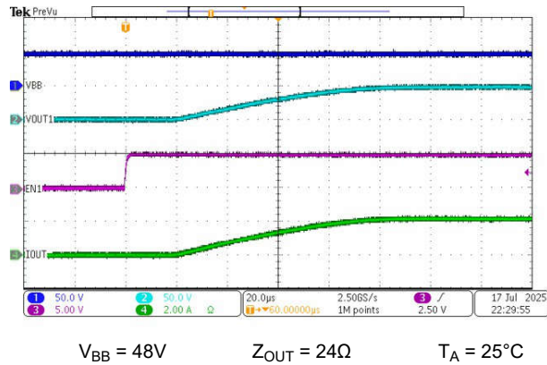
Figure 8-4. Turn-on with Resistive Load
