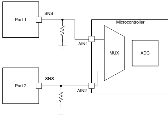
Figure 7-12. SNS Sharing Across Multiple Devices Method 1
