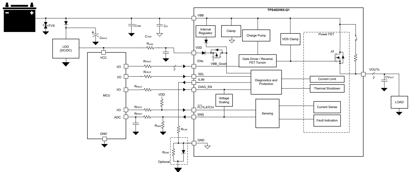
Figure 8-1. Typical Application Diagram for GPIO version
