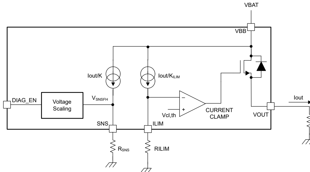
Figure 7-3. Current-Sense and Current-Limit Block Diagram
