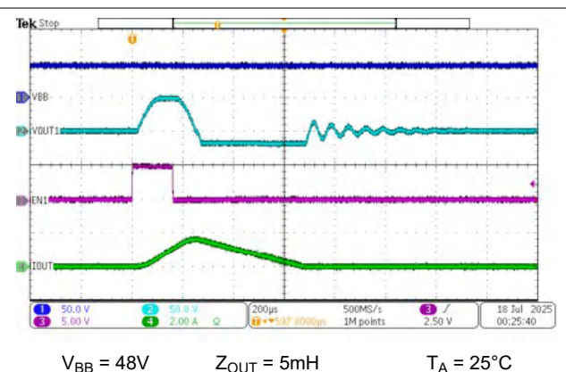
Figure 8-3. Inductive Load Discharge
