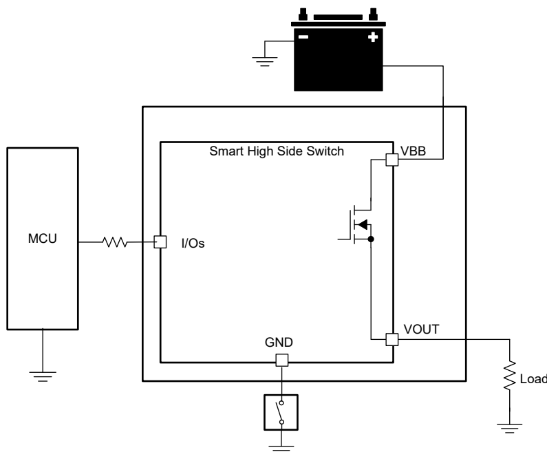
Figure 7-17. Loss of Device GND
