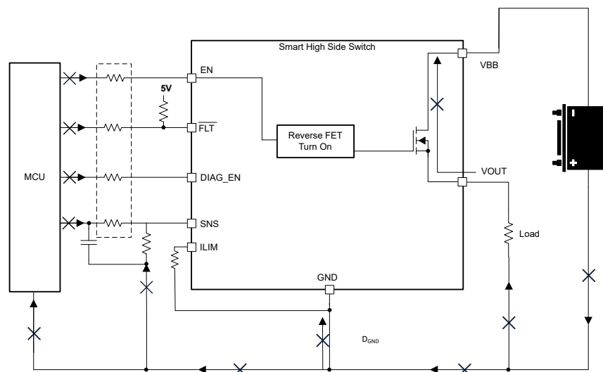
Figure 7-20. Reverse Protection With Block Diode
