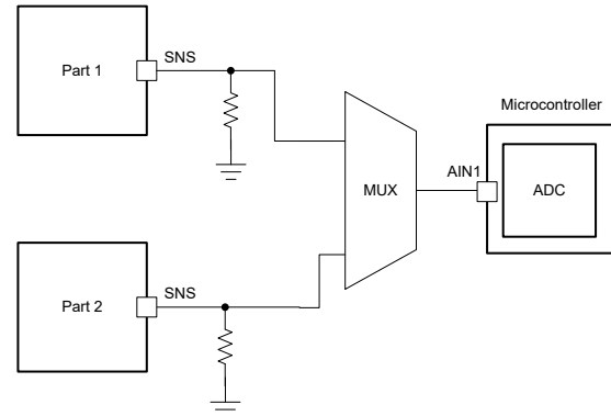
Figure 7-13. SNS Sharing Across Multiple Devices Method 2
