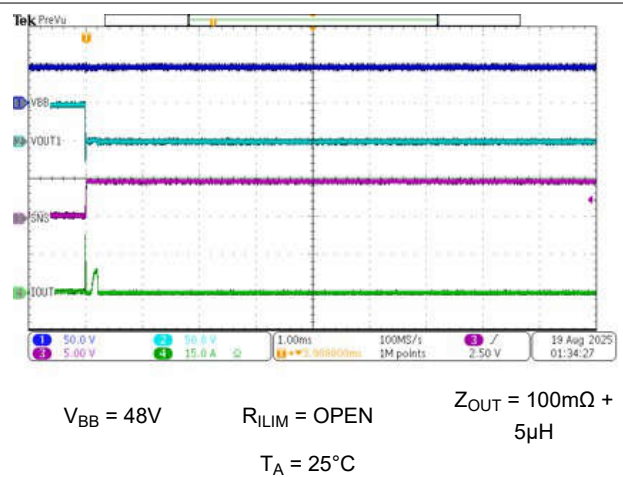
Figure 8-7. Hot Short (Latch behavior)
