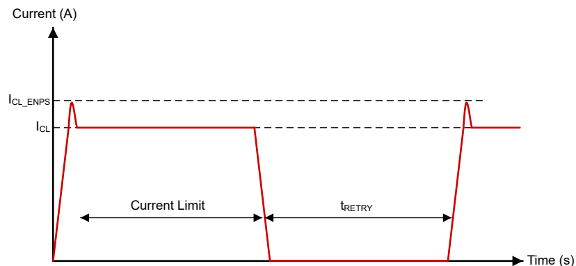
Figure 7-4. Enable Into Short Current Limit (auto-retry)
