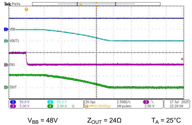
Figure 8-5. Turn-off with Resistive Load
