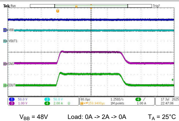
Figure 8-6. Load Transient Behavior
