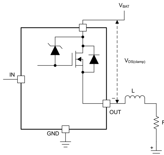
Figure 7-8. Drain-to-Source Clamping Structure
