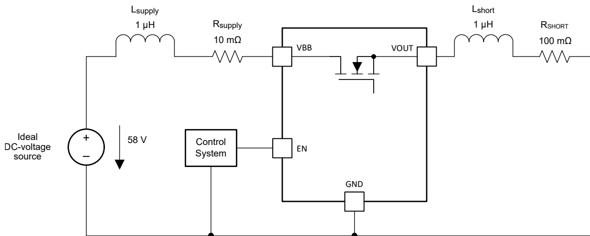
Figure 7-7. Equivalent Test Circuit
