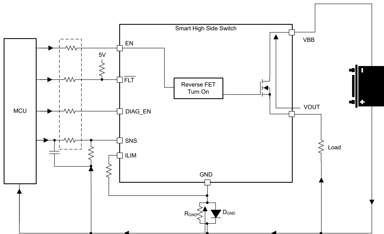
Figure 7-22. MCU I/O Protections
