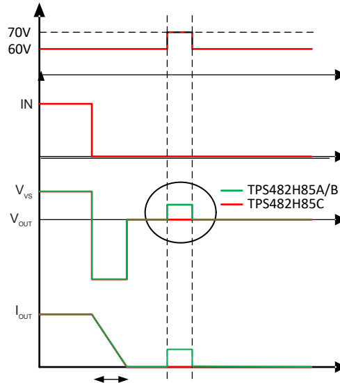
Figure 7-11. Inductive Load Switching-Off Differences Between A, B and C Variants
