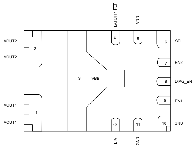
Figure 5-1. CHU Package 12-Pin VQFN-HR Bottom View
