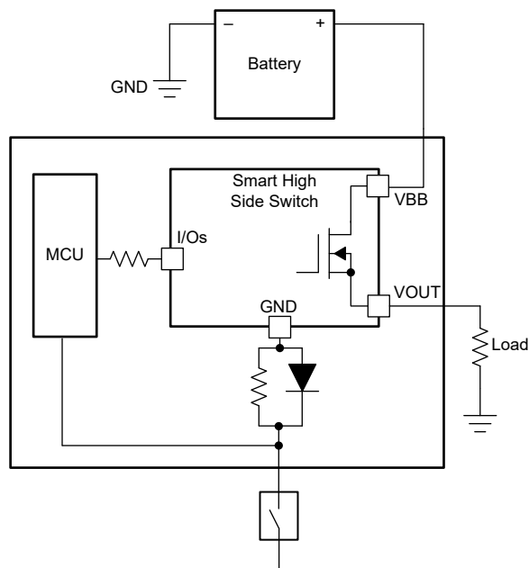
Figure 7-18. Loss of Module GND
