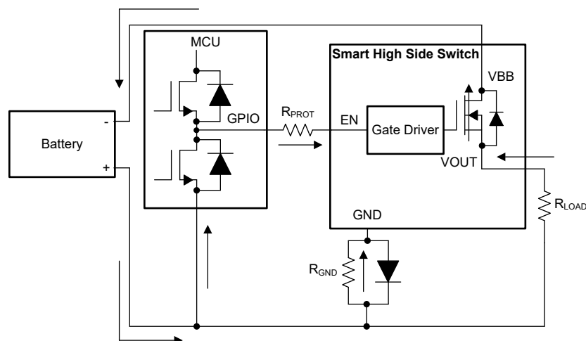
Figure 7-15. Reverse Battery Circuit
