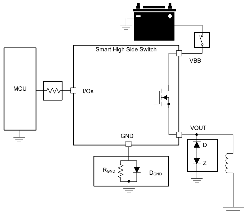
Figure 7-19. Loss of Battery
