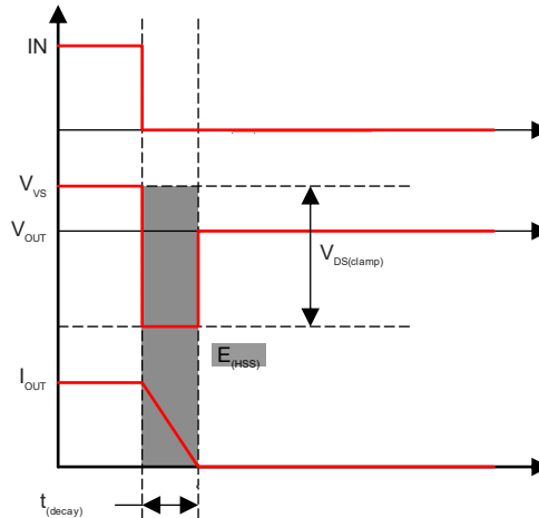
Figure 7-9. Inductive Load Switching-Off Diagram
