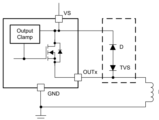
Figure 7-10. Protection With External Circuitry
