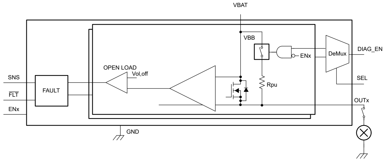
Figure 7-14. Open-Load Detection in Off-State
