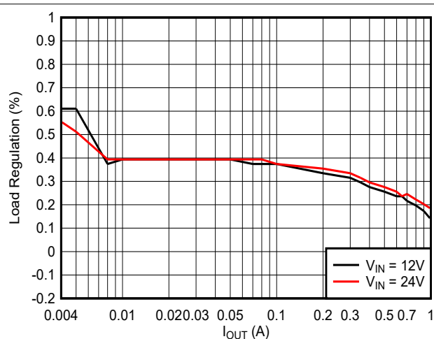
Figure 7-9. TPS561300EVM Load Regulation
