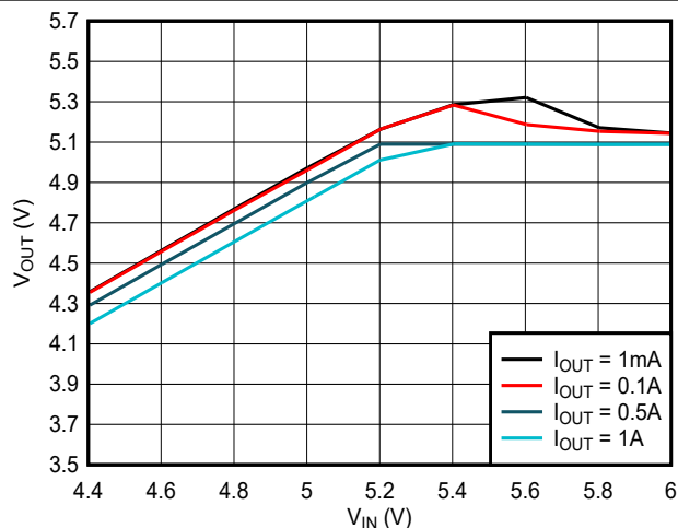
Figure 7-11. TPS561300EVM Drop Out
