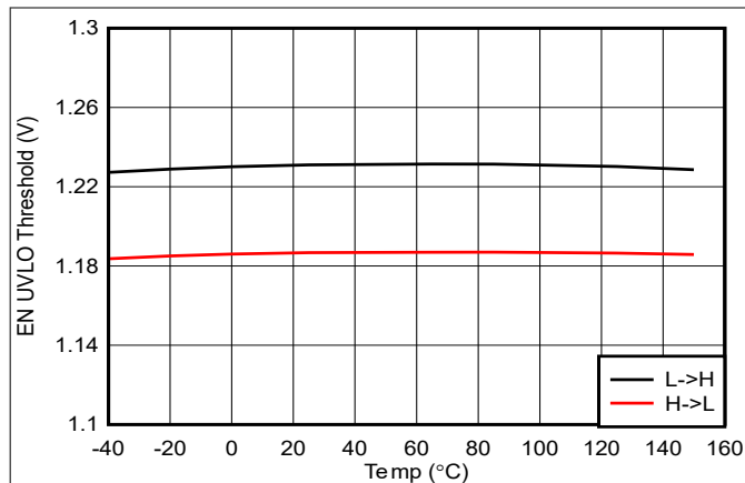
Figure 5-7. EN Threshold vs Junction Temperature
