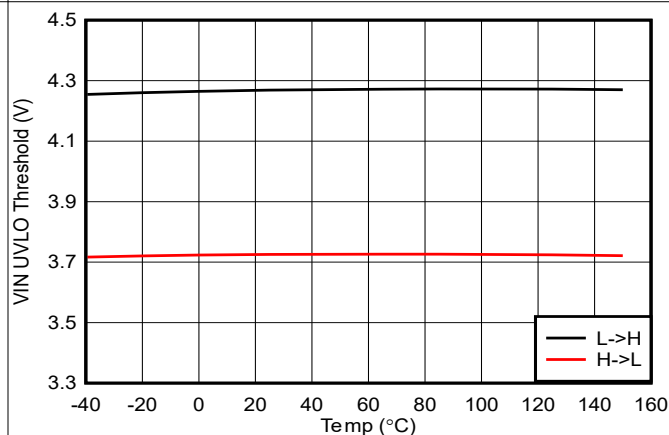
Figure 5-6. VIN UVLO Threshold vs Junction Temperature
