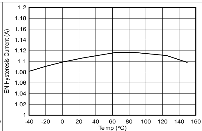
Figure 5-8. EN Hysteresis Current vs Junction Temperature
