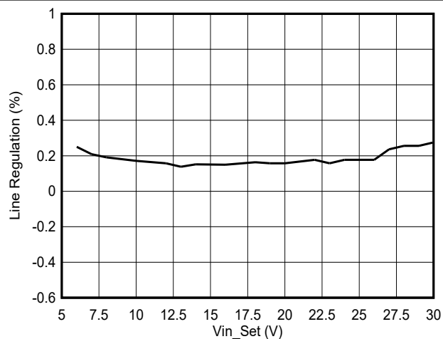
Figure 7-10. TPS561300EVM Line Regulation, I_{OUT} = 1A
