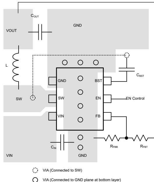
Figure 7-12. Board Layout
