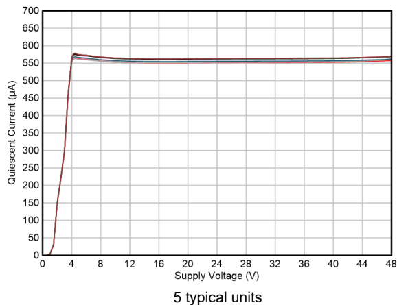
Figure 5-25. Quiescent Current vs Supply Voltage
