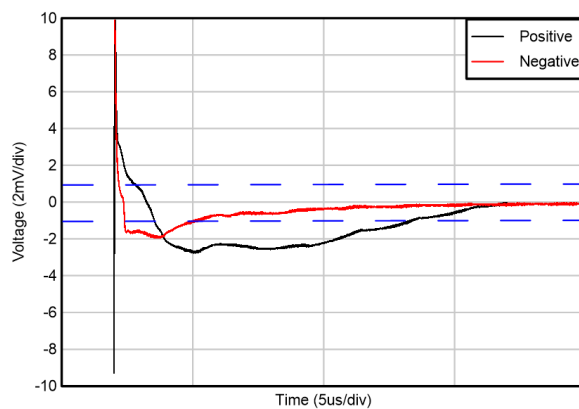
Figure 5-38. Settling Time
