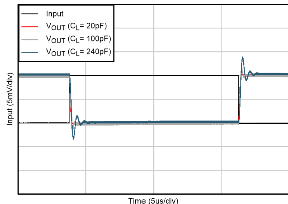
Figure 5-31. Positive Overload Recovery
