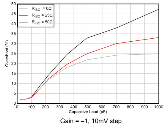
Figure 5-36. Small-Signal Overshoot vs Capacitive Load
