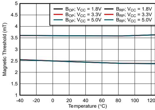
Figure 6-3. 3.5mT B_{OP} : Thresholds vs Temperature
