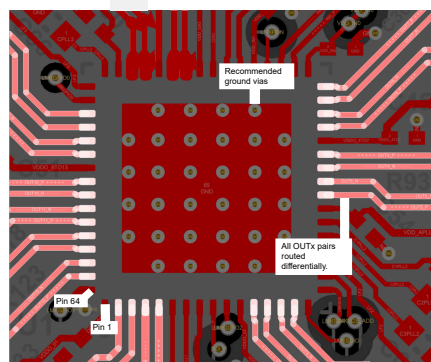
Figure 9-6. PCB Layout Example for LMK5B33216, Top Layer
