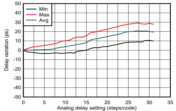
Figure 6-21. SYSREF/1PPS Delay Linearity vs. Analog Delay Code 2
