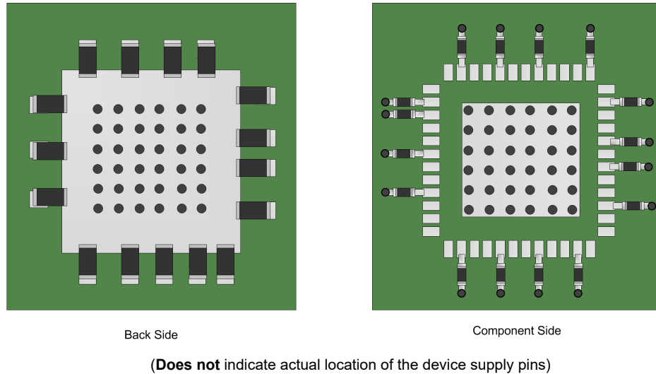
Figure 9-5. Generalized Placement of Power Supply Bypass Capacitors
