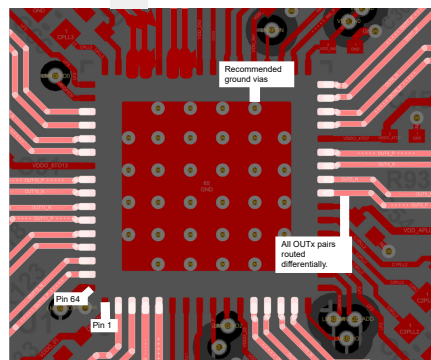
Figure 9-6. PCB Layout Example for LMK5B33216, Top Layer
