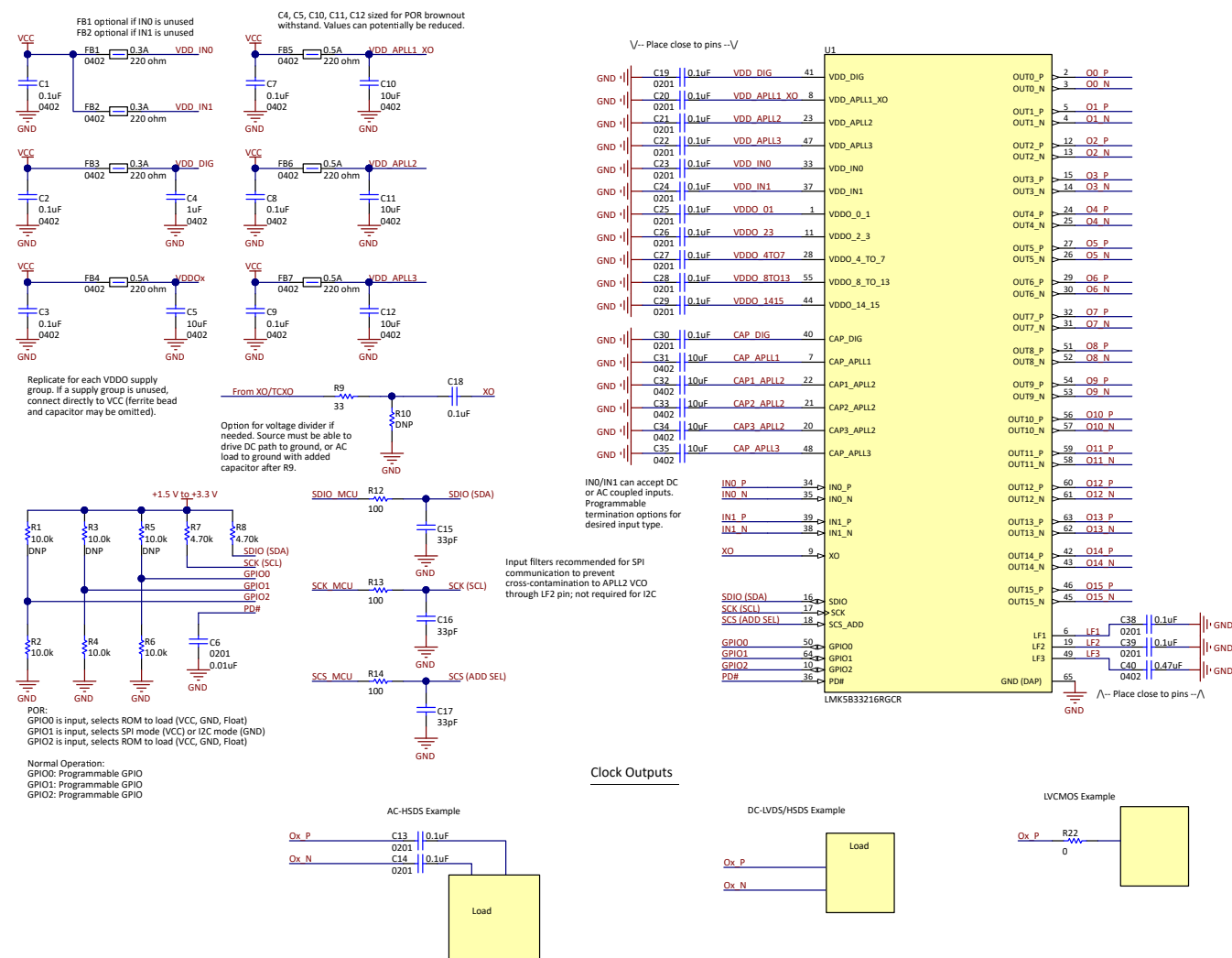
Figure 9-4. Typical Application Example
