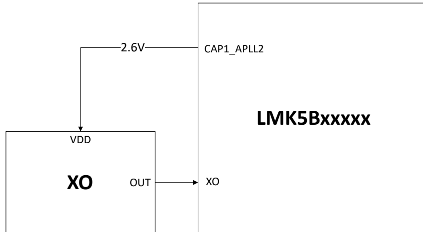
Figure 9-3. Supplying XO Input With CAP1_APLL2
