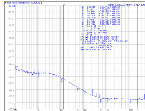
Figure 6-9. 156.25MHz HSDS Output From BAW APLL
