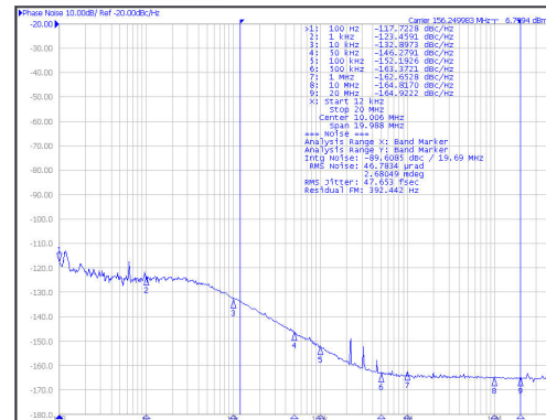
Jitter = 47fs RMS (12kHz to 20MHz) f BAW APLL = 2500MHz (BAW APLL post-divider = 8, div2 enabled) Figure 6-9. 156.25MHz HSDS Output From BAW APLL
