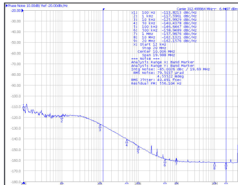
Jitter = 41fs RMS (12kHz to 20MHz) f BAW APLL = 2500MHz (BAW APLL post-divider = 8) Figure 6-8. 312.5MHz HSDS Output From BAW APLL
