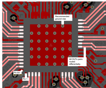
Figure 9-6. PCB Layout Example for LMK5B33414, Top Layer
