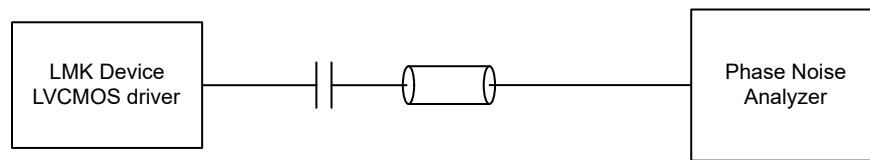
Figure 7-4. LVCMOS Output Phase Domain Test Configuration
