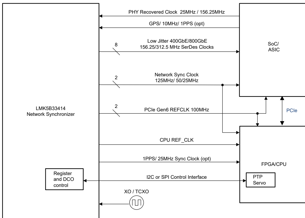
LMK5B33414 Typical System Block Diagram
