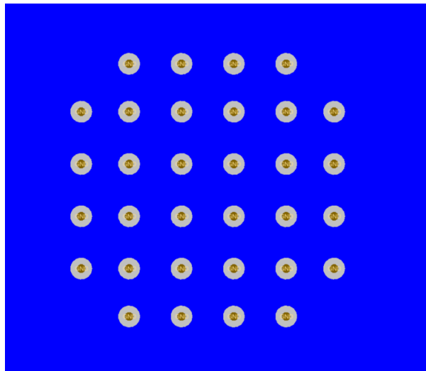
Figure 9-7. PCB Layout Example for LMK5B33414, Bottom Layer
