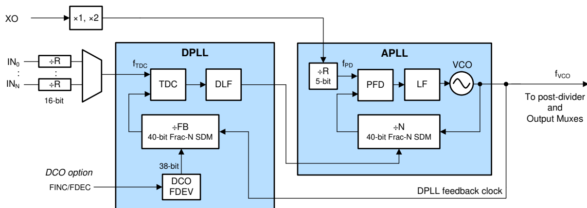
Figure 8-23. PLL Architecture
