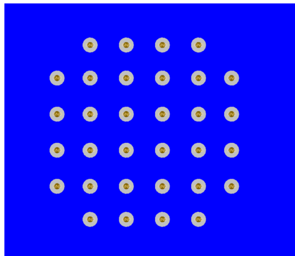
Figure 9-7. PCB Layout Example for LMK5B33414, Bottom Layer
