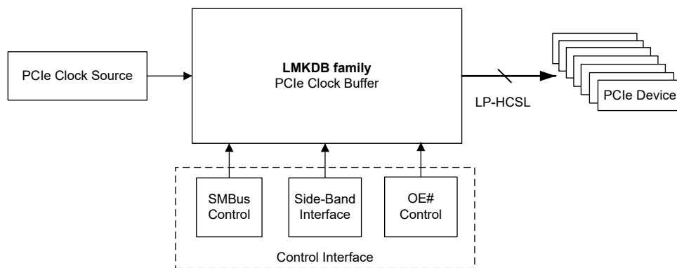
Typical Application
