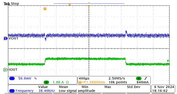
Device type = 1A 3.3V output Mode = FPWM F_{sw} = 2\text{MHz}
