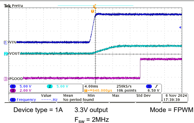
Figure 8-16. Start-up
