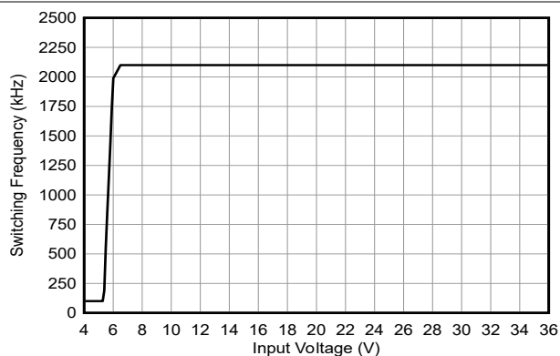
Figure 8-15. Switching Frequency vs Input Voltage
