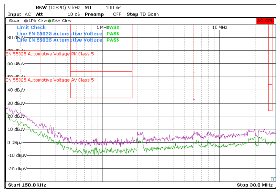
V_{OUT} = 5\text{V} F_{SW} = 2\text{MHz} I_{OUT} = 1\text{A} Frequency span: 150kHz to 30MHz
