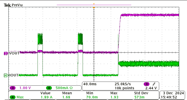
Device type = 1A 3.3V output Mode = FPWM F_{sw} = 2\text{MHz}
