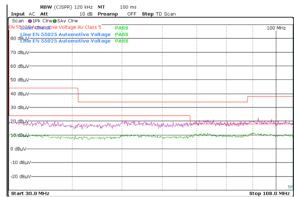
V_{OUT} = 5\text{V} F_{SW} = 2\text{MHz} I_{OUT} = 1\text{A} Frequency span: 30MHz to 108MHz
