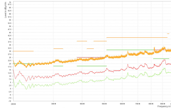
Figure 8-30. Radiated EMI versus CISPR25 Limits (Yellow: Peak Signal, Red: Quasipeak Signal, Green: Average Signal), Vertical Biconical Antenna, LMR60410QEVm
