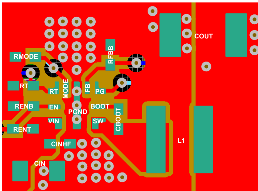
Figure 8-36. Example Layout
