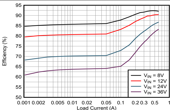
Figure 8-5. Efficiency
