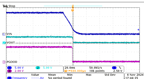
Figure 8-15. Shutdown
