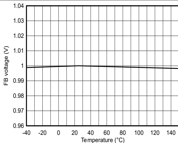
Figure 6-9. Feedback voltage accuracy
