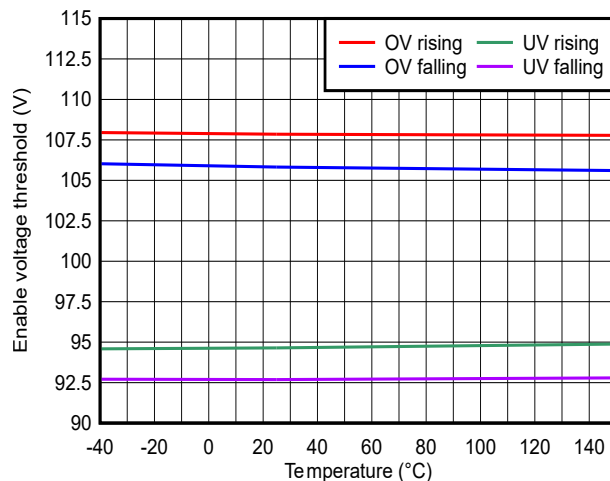
Figure 6-12. PGOOD thresholds
