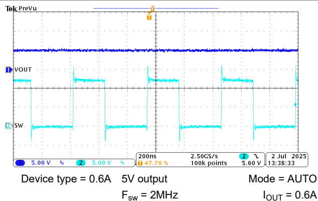
Figure 8-20. Steady State Waveform
