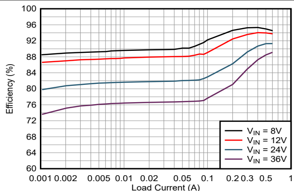
Figure 8-3. Efficiency
