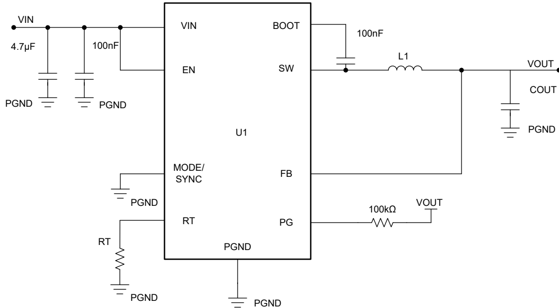
Figure 8-30. Example Application Circuit
