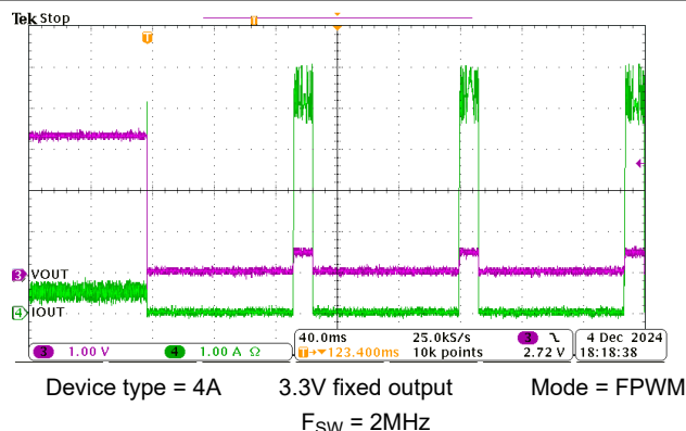
Figure 8-21. Short-Circuit Applied
