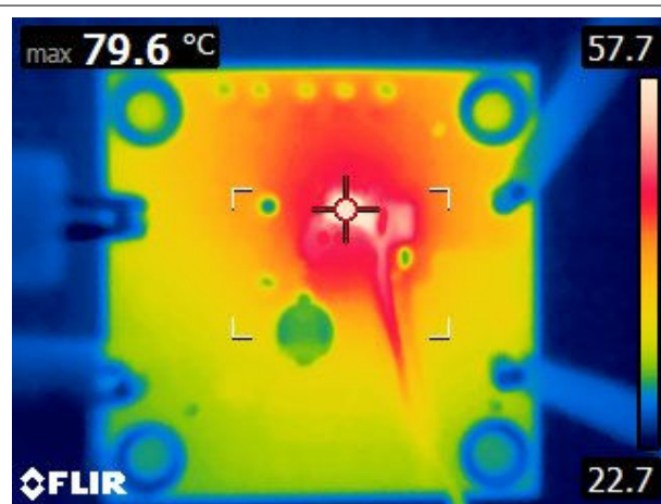
Figure 8-21. Short-Circuit Applied
