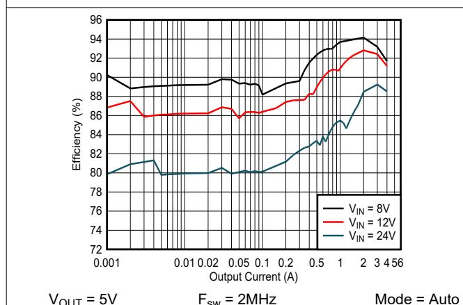
Figure 8-4. Efficiency
