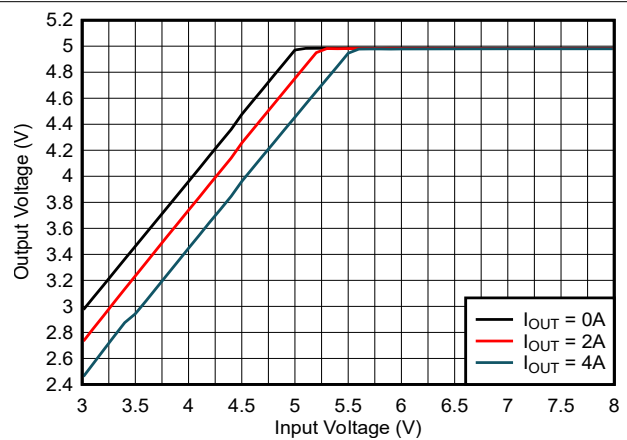
Figure 8-11. Dropout
