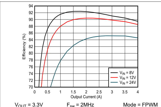
Figure 8-3. Efficiency
