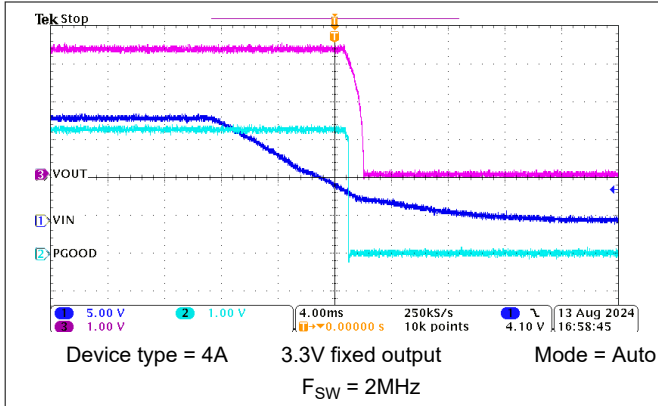
Figure 8-20. Shutdown Operation
