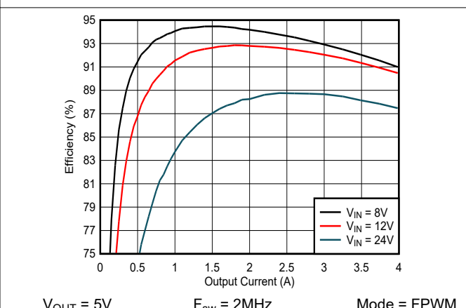
Figure 8-5. Efficiency
