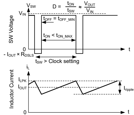
Figure 7-11. Dropout Waveforms
