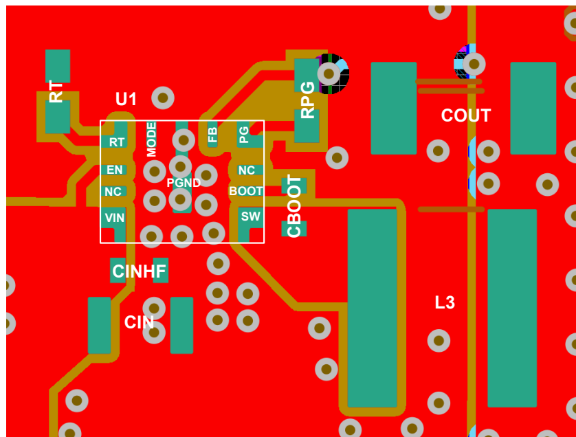
Figure 8-35. Recommended Layout Example for RBM Package (3.5mm × 2.5mm)
