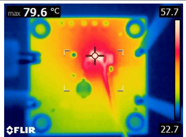
Figure 8-21. Short-Circuit Applied
