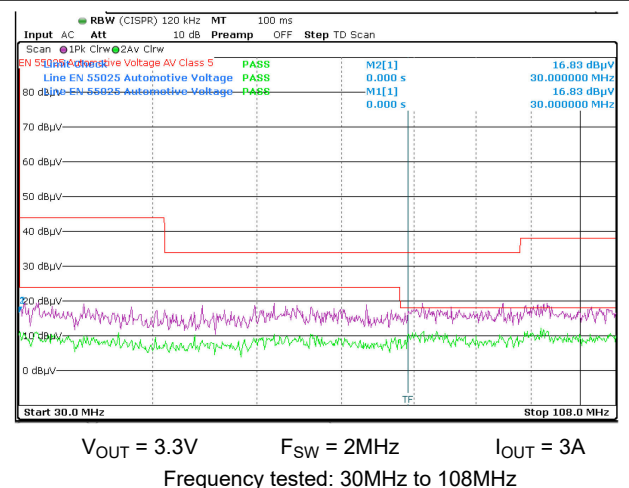
Figure 8-25. Conducted EMI versus CISPR25 Limits (Purple: Peak Signal, Green: Average Signal), LMR60440QEV
