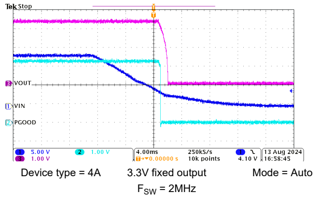
Figure 8-20. Shutdown Operation
