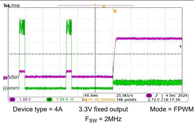
Figure 8-22. Short-Circuit Recovery
