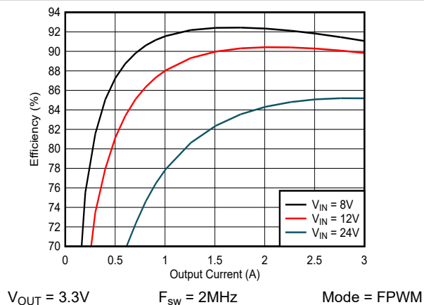
Figure 8-3. Efficiency
