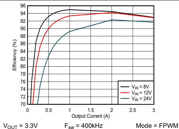
Figure 8-5. Efficiency
