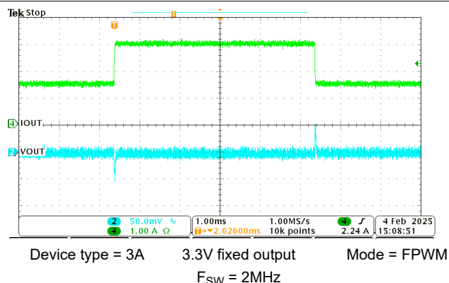
Figure 8-16. 1.5A to 3A Load Transient
