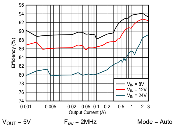
Figure 8-6. Efficiency
