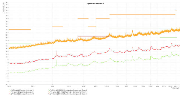
Figure 8-32. Radiated EMI Bicon Horizontal versus CISPR25 Limits, LMR60440QEV
