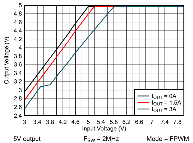
Figure 8-11. Dropout
