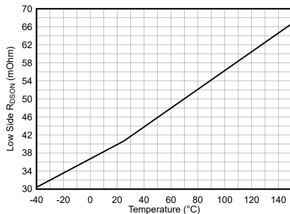
Figure 6-4. Low Side MOSFET R_{DS-ON}
