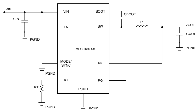
Simplified Schematic – Fixed Output
