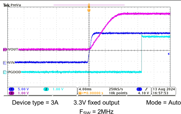
Figure 8-17. Start-Up Operation
