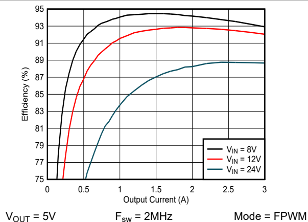
Figure 8-7. Efficiency
