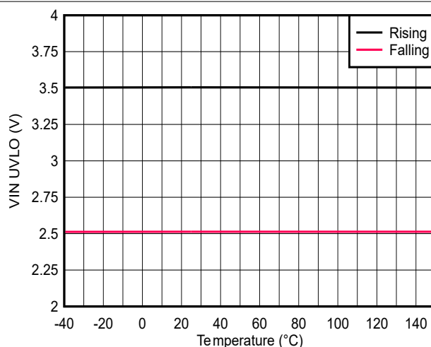
Figure 6-10. Input Voltage UVLO - B Variant
