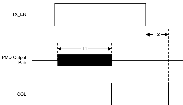
Figure 6-15. 10BASE-Tc Jabber Timing
