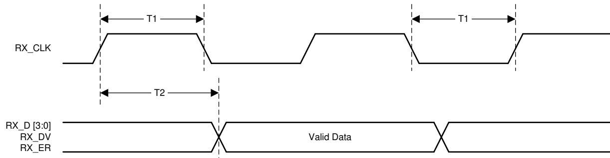
Figure 6-8. 10Mbps Receive Timing
