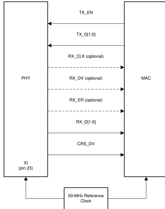
Figure 7-5. RMII Follower Signaling
