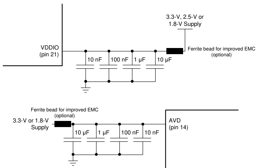
Figure 9-5. Power Connections
