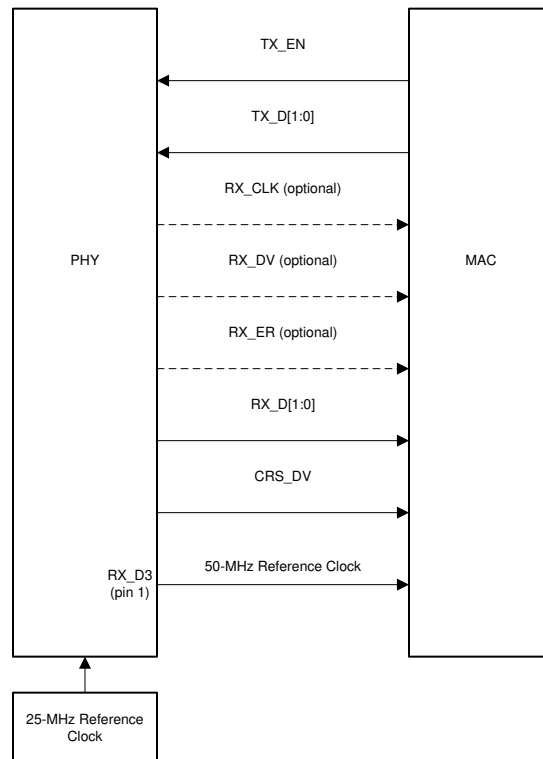
Figure 7-6. RMII Leader Signaling
