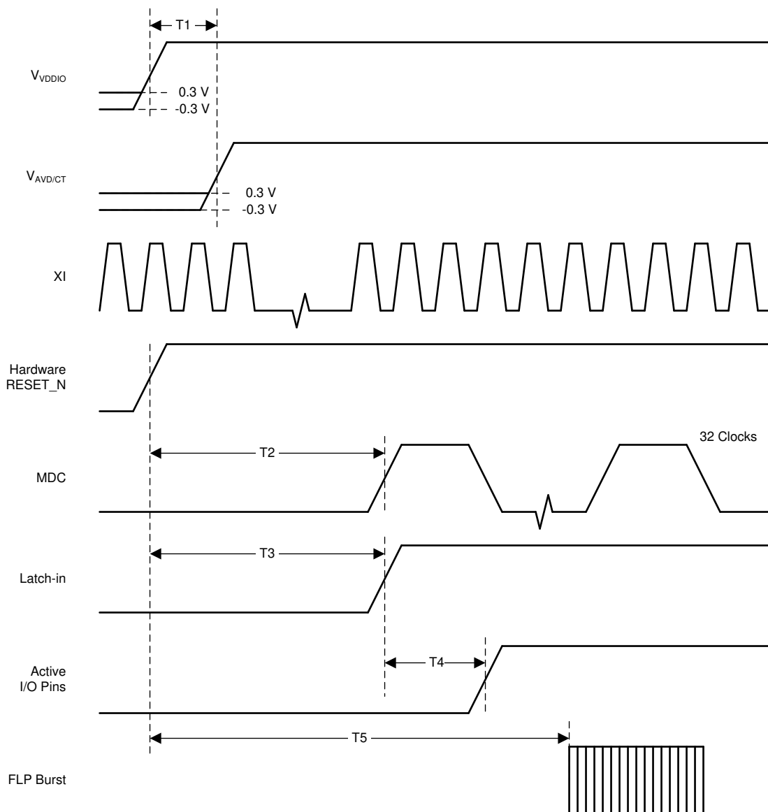
Figure 6-1. Power-Up Timing
