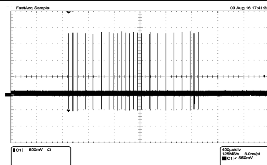
Figure 6-19. 10BASE-Tc Link Pulse Waveform
