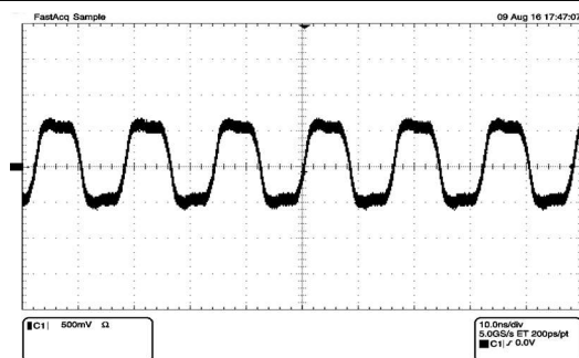
Figure 6-18. 100BASE-TX PMD Eye Waveform
