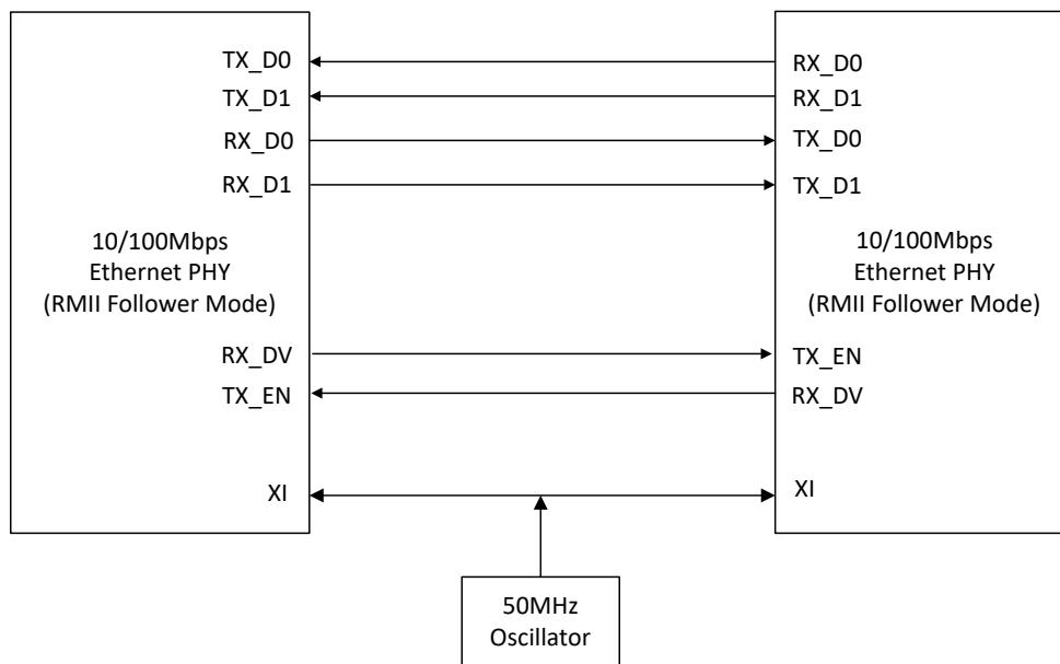
Figure 7-8. RMI Repeater Mode: Follower-Follower
