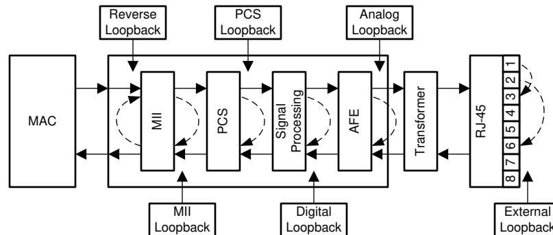
Figure 7-10. Loopback Test Modes
