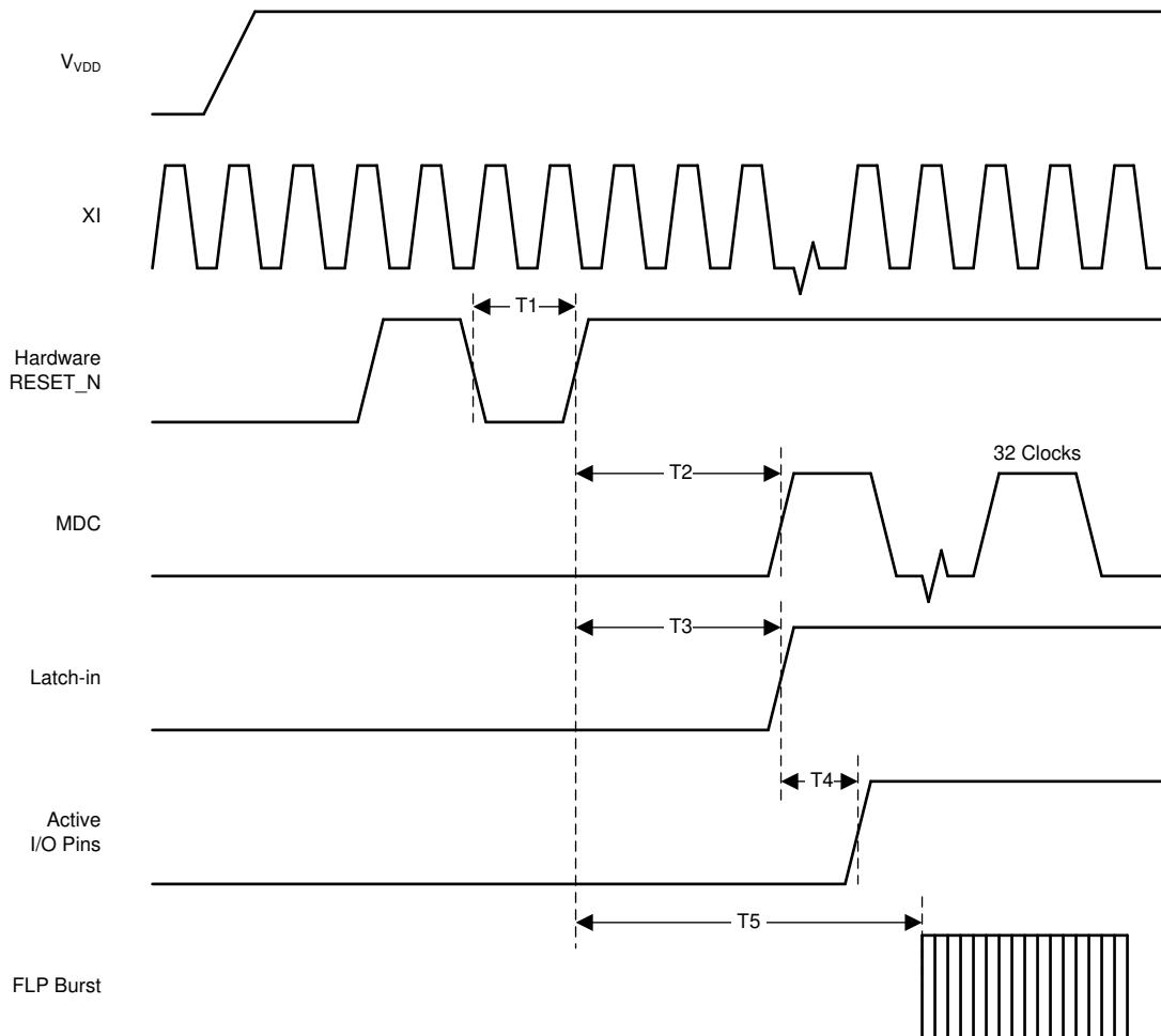
Figure 6-3. Reset Timing
