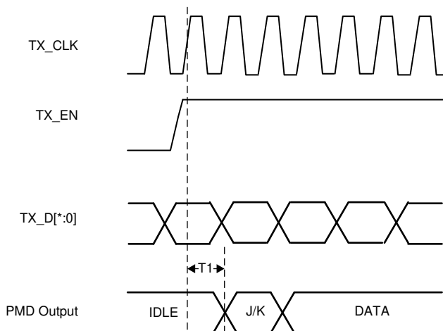
Figure 6-16. 100BASE-TX Transmit Latency Timing
