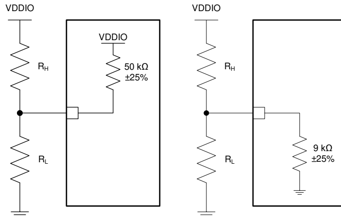
Figure 7-12. Bootstrap Circuits
