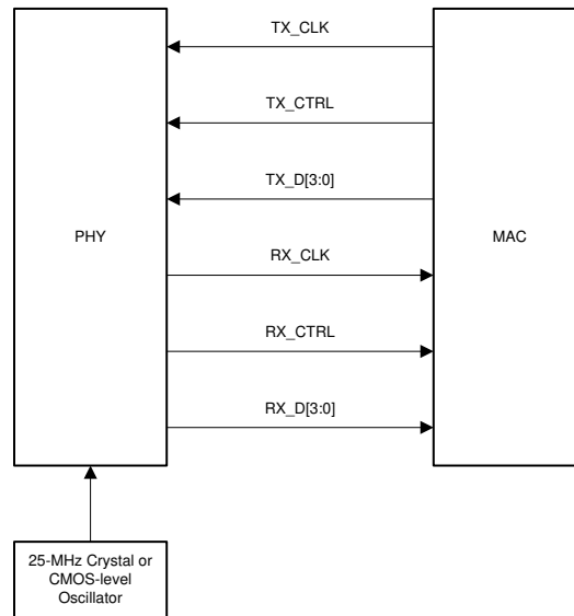
Figure 7-9. RGMII Signaling
