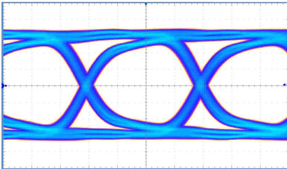
Figure 6-3. Eye Diagram at 4-Gbps FPD-Link III Forward Channel Rate From Serializer Output Scale: 100 mV/DIV Horizontal Scale: 62.5 ps/DIV
