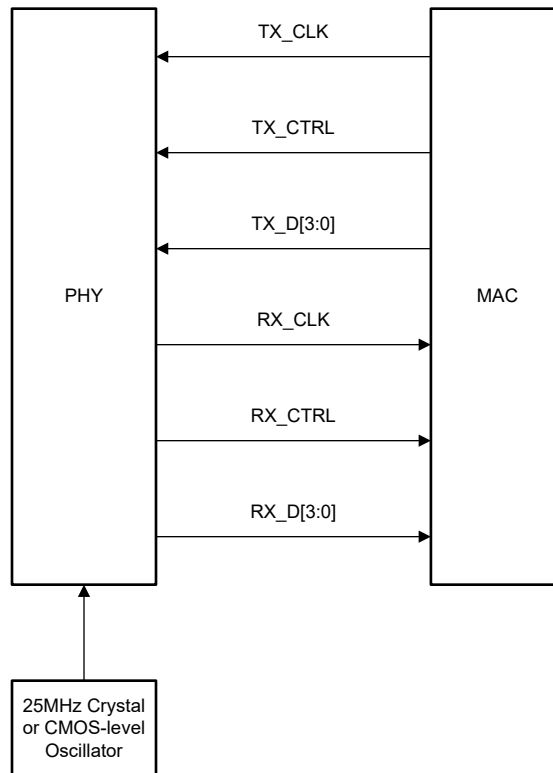
Figure 7-16. RGMII Connections
