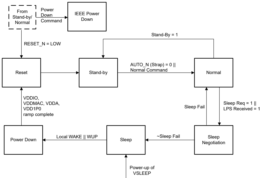
Figure 7-11. Power State Diagram
