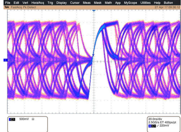
Figure 9-8. MDI IDLE Stream (Variable Persistence)
