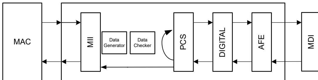
Figure 7-10. Reverse Loopback Without Data Generator
