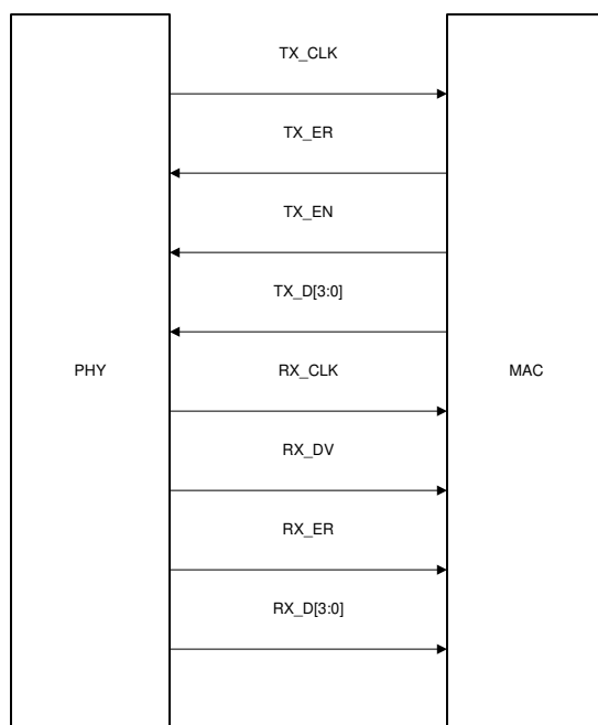
Figure 7-14. MII Signaling
