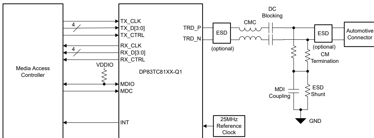
Figure 9-5. Typical Application (RGMII)
