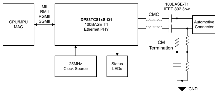
Simplified Schematic
