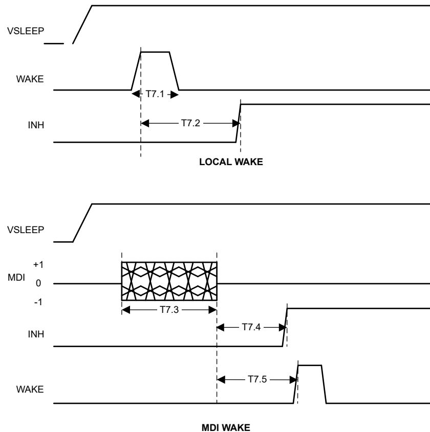
Figure 6-9. WAKE Timing
