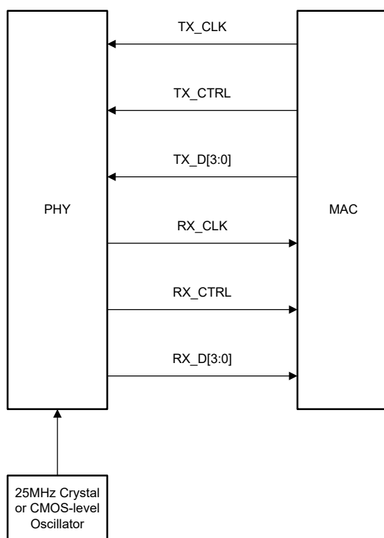
Figure 7-16. RGMII Connections
