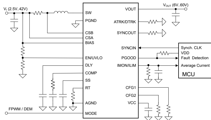
Typical Application
