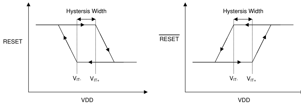
Figure 7-1. Hysteresis Diagram
