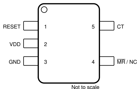
Figure 5-1. DBV Package 5-Pin SOT-23 TPS3840PL, Figure 5-2. DBV Package 5-Pin SOT-23 TPS3840PH Top View
