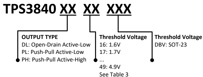
Figure 4-1. Device Nomenclature
