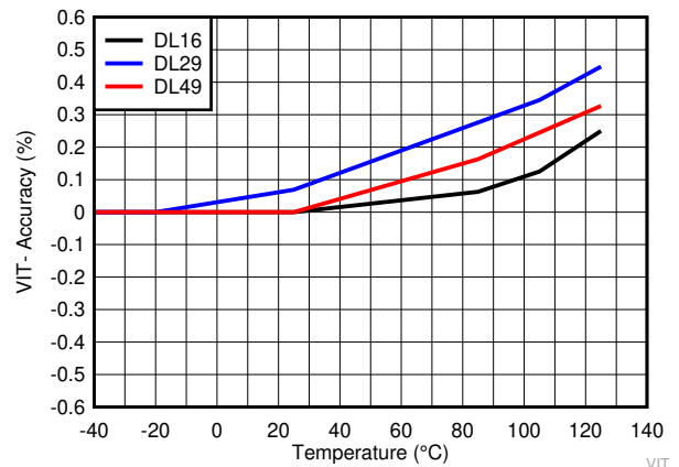
Figure 6-7. Negative-going Input Threshold Accuracy over Temperature for TPS3840DLXX
