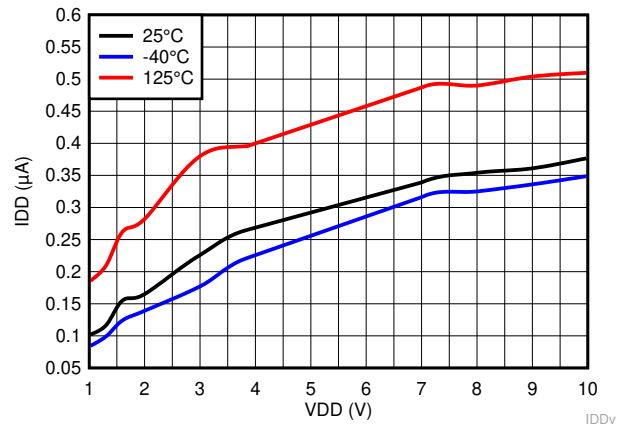
Figure 6-5. Supply Current vs Supply Voltage for TPS3840PL49
