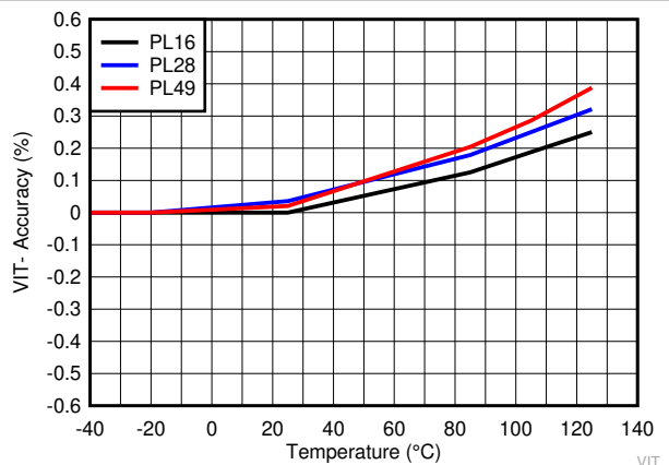
Figure 6-8. Negative-going Input Threshold Accuracy over Temperature for TPS3840PLXX
