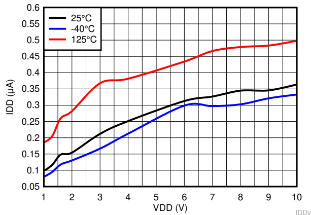
Figure 6-4. Supply Current vs Supply Voltage for TPS3840DL49
