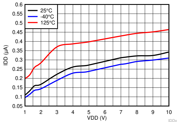
Figure 6-6. Supply Current vs Supply Voltage for TPS3840PH49
