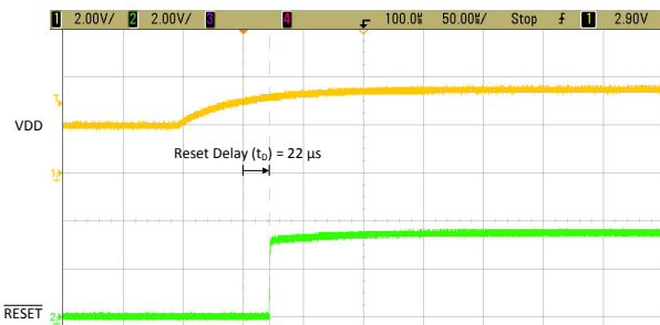
Figure 8-7. TPS3840EVM RESET Time Delay ( t_D ) with No Capacitor
