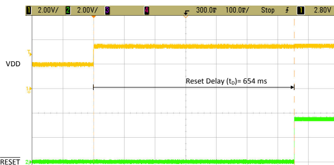
Figure 8-9. TPS3840EVM RESET Time Delay ( t_D ) with 1-μF Capacitor
