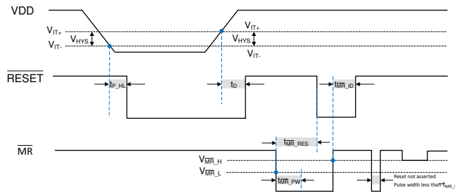
Figure 7-3. Timing Diagram \overline{\text{MR}} and \overline{\text{RESET}} (TPS3840DL)
