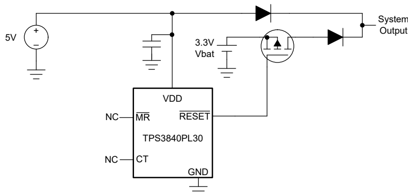
Figure 8-6. Voltage Monitor with Back-up Battery Switchover Solution
