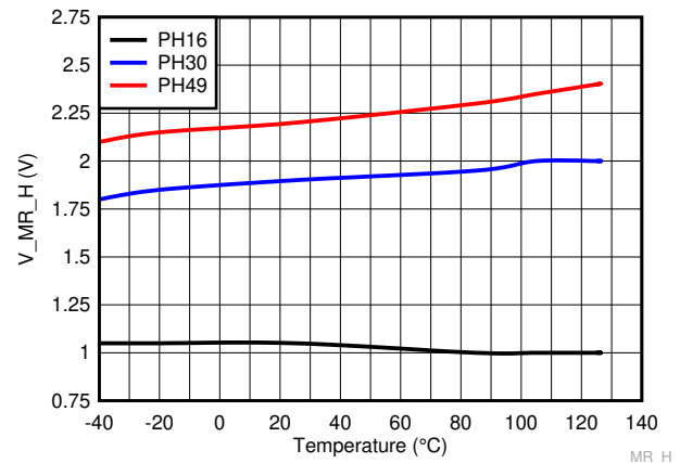
Figure 6-31. Manual Reset Logic High Voltage Threshold over Temperature for TPS3840PHXX
