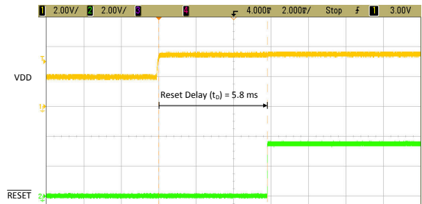
Figure 8-8. TPS3840EVM \overline{\text{RESET}} Time Delay ( t_D ) with 0.01- \mu\text{F} Capacitor
