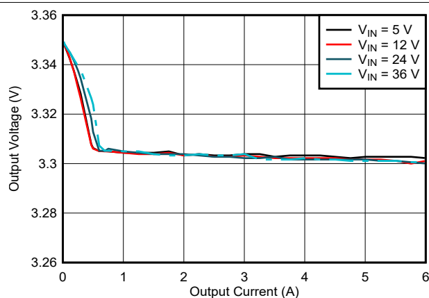
Figure 8-23. LM634x0-Q1 Load and Line Regulation
