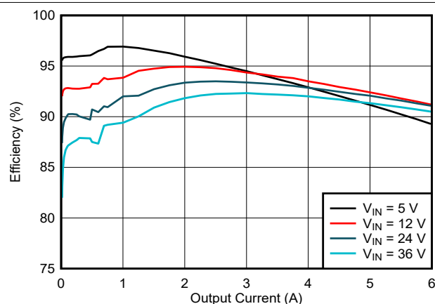
Figure 8-22. LM634x0-Q1 Efficiency
