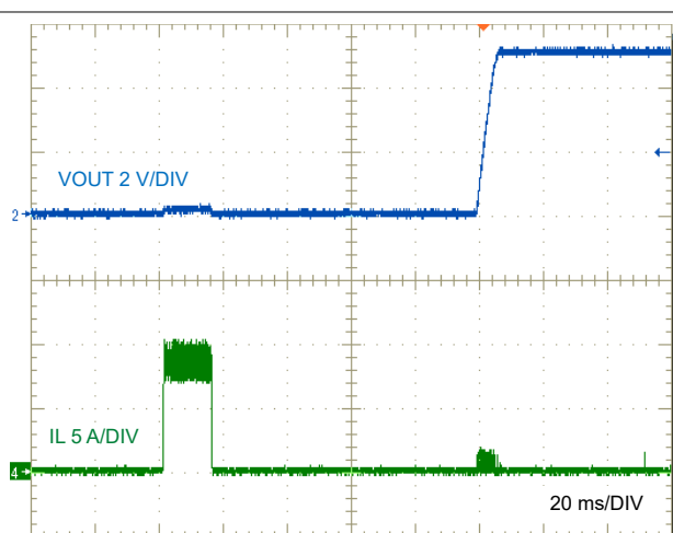
Figure 7-11. Short-Circuit Recovery
