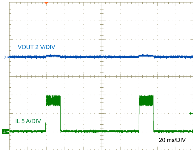
Figure 8-28. LM634x0-Q1 Short-Circuit Hiccup
