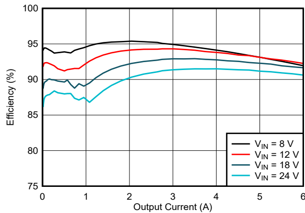
Figure 8-3. LM634x0-Q1 Efficiency
