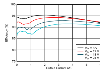
Efficiency, V_{\text{OUT}} = 5\text{V} , f_{\text{SW}} = 2.1\text{MHz} , LM63460-Q1
