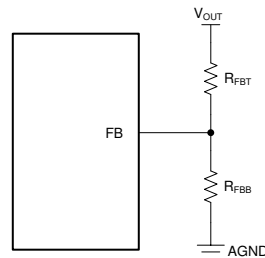
Figure 7-6. Setting Output Voltage for Adjustable Output Variant
