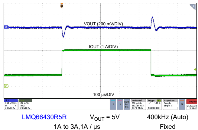
Figure 8-9. Load Transient
