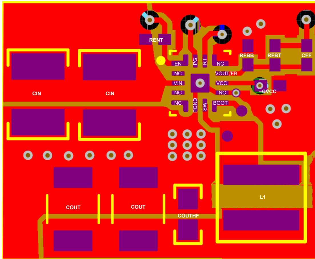
Figure 8-13. Example Layout
