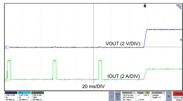
Figure 7-12. Hiccup Exit
