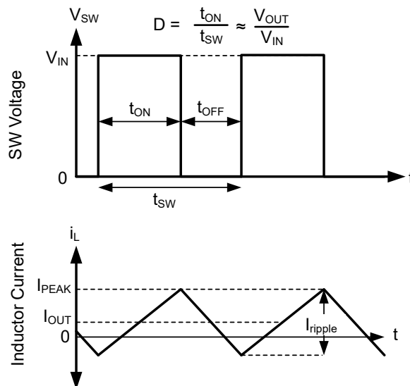
Figure 7-16. FPWM Mode Operation
