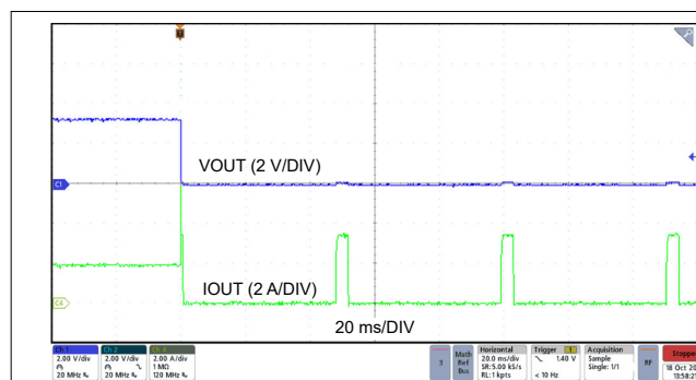
Figure 7-11. Hiccup Entry
