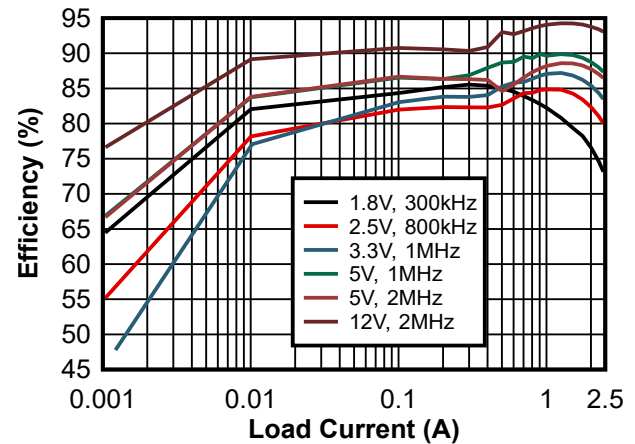
Figure 8-6. 24VIN Efficiency (Log)
