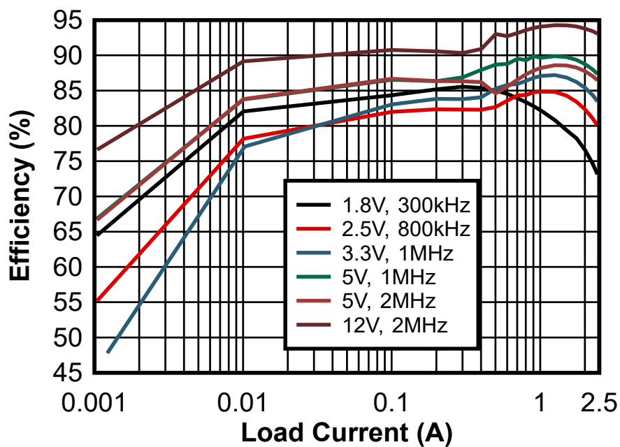
Efficiency vs Output Current V_{IN} = 24V
