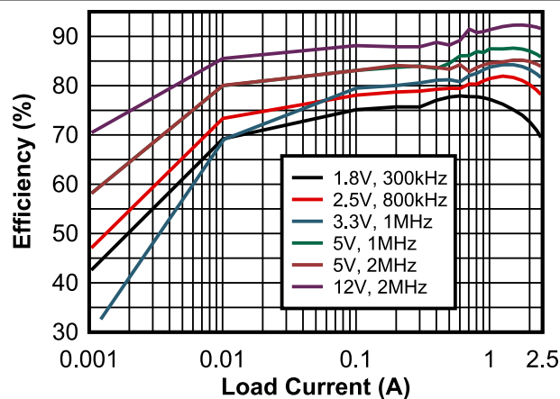
Figure 8-9. 36VIN Efficiency (Log)
