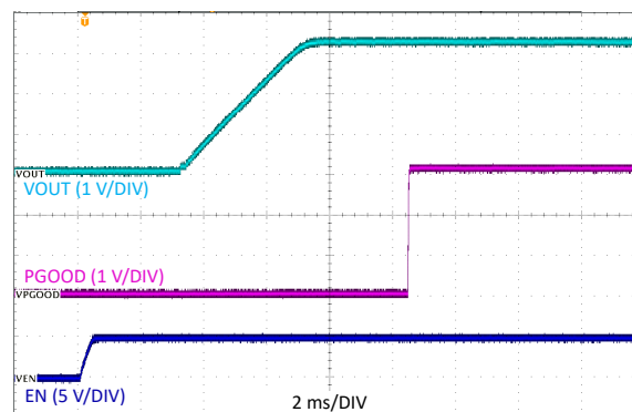
Figure 7-4. Enable Start-Up V_{IN} = 24V , V_{OUT} = 3.3V , I_{OUT} = 2.5A I_{OUT} = 1.5A
