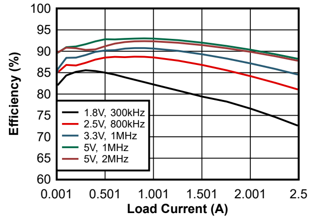
Figure 8-4. 12VIN Efficiency (Linear)
