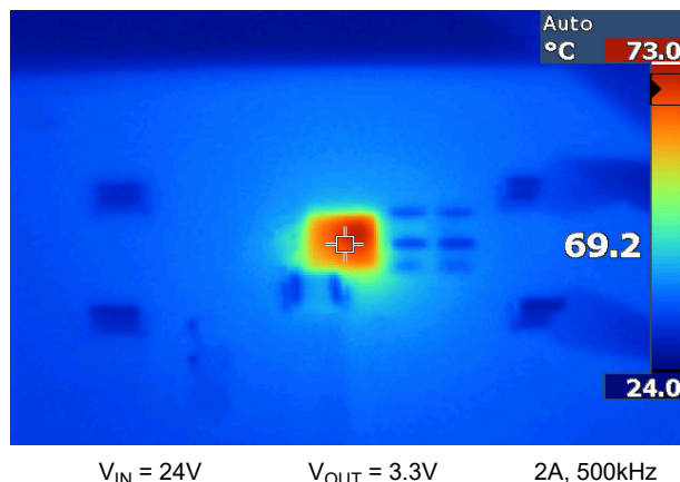
Figure 8-17. EVM Thermal Performance
