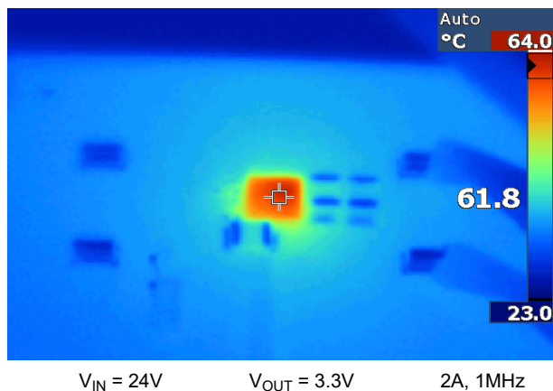
Figure 8-18. EVM Thermal Performance
