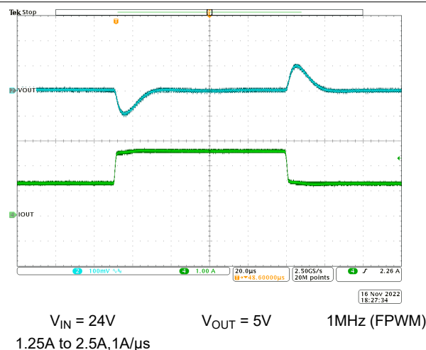
Figure 8-13. Load Transient
