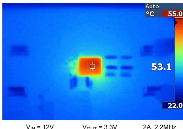
Figure 8-16. EVM Thermal Performance
