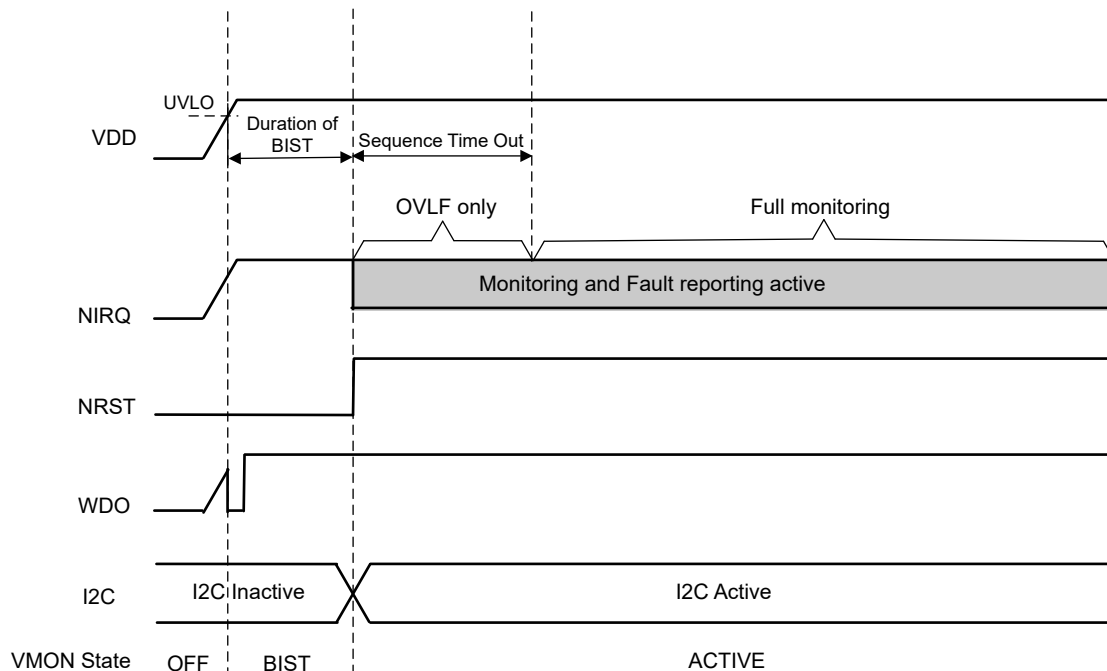
Figure 7-31. TPS389C03-Q1 Power ON Signaling and Internal States
