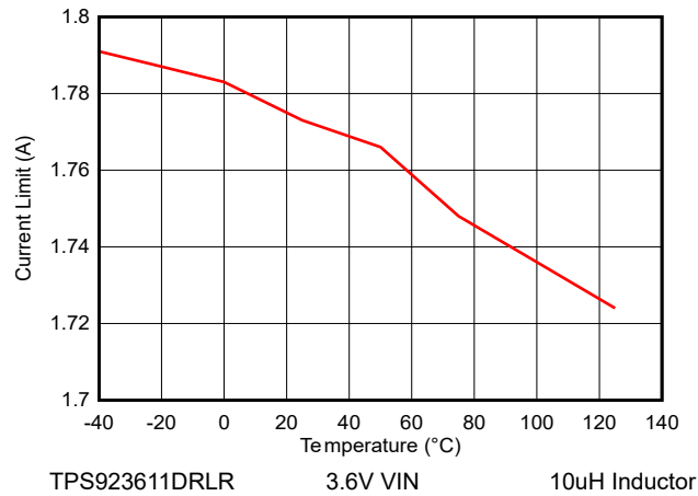
Figure 6-13. Current Limit vs Temperature
