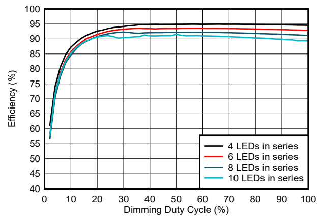
TPS923612DRVVR 10uH Inductor 5V Input Voltage 120mA IOUT at 100% Dutycycle
