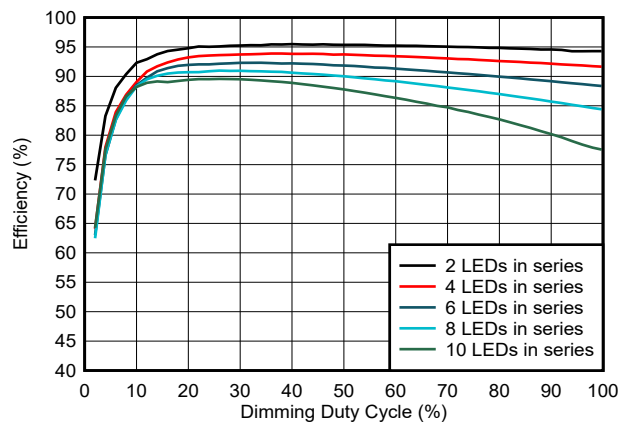
TPS923612DRVVR 10uH Inductor 3.6V Input Voltage 120mA IOUT at 100% Dutycycle
