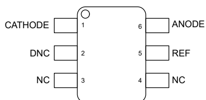
Figure 5-3. DRL Package, 6-Pin SOT-563, TLA431 (Top View)
