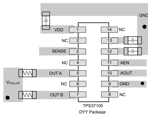
Figure 8-3. TPS37100 Recommended Layout
