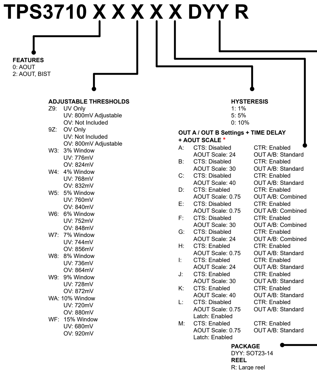
Figure 4-1. Device Naming Convention (Adjustable Threshold Variant)
