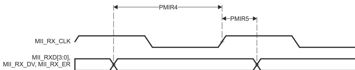
Figure 6-108. PRU_ICSSG MII[x]_RXD[3:0], MII[x]_RX_DV, and MII[x]_RX_ER Timing
