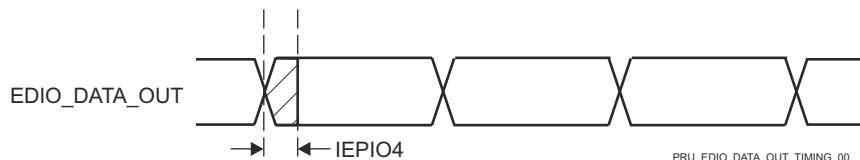
Figure 6-101. PRU_ICSSG IEP Digital IOs Timing Requirements
