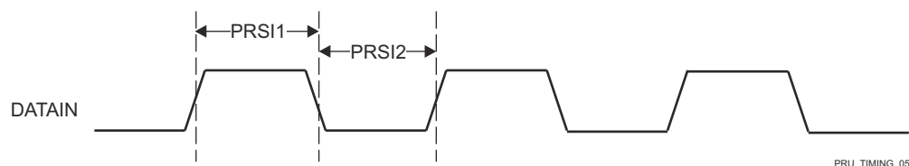
Figure 6-93. PRU_ICSSG PRU Shift In Timing
