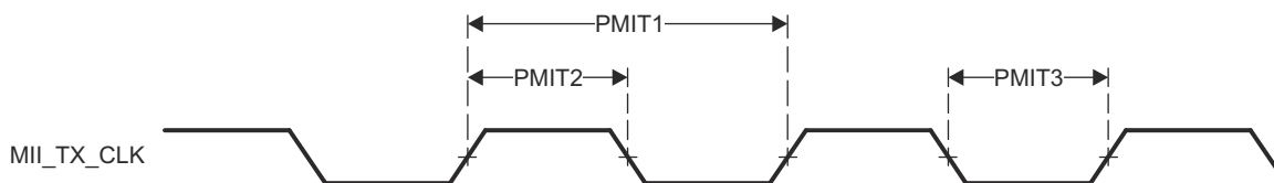
Figure 6-109. PRU_ICSSG MII[x]_TX_CLK Timing
