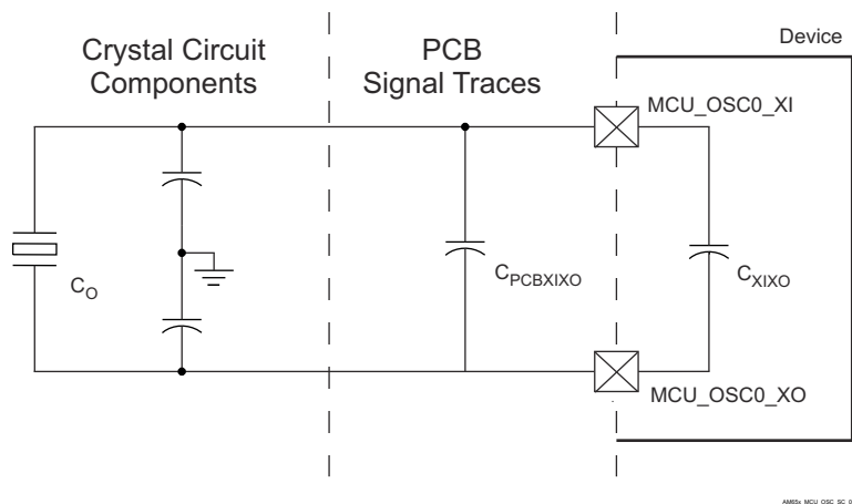
Figure 6-20. Shunt Capacitance
