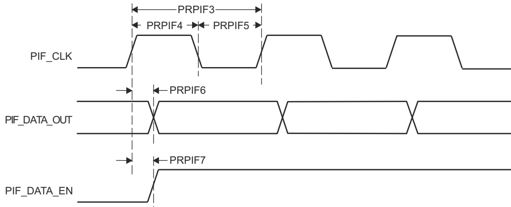
Figure 6-98. PRU_ICSSG PRU Peripheral Interface Switching Characteristics
