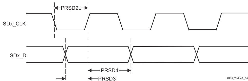
Figure 6-96. PRU_ICSSG PRU SD_CLK Rising Active Edge
