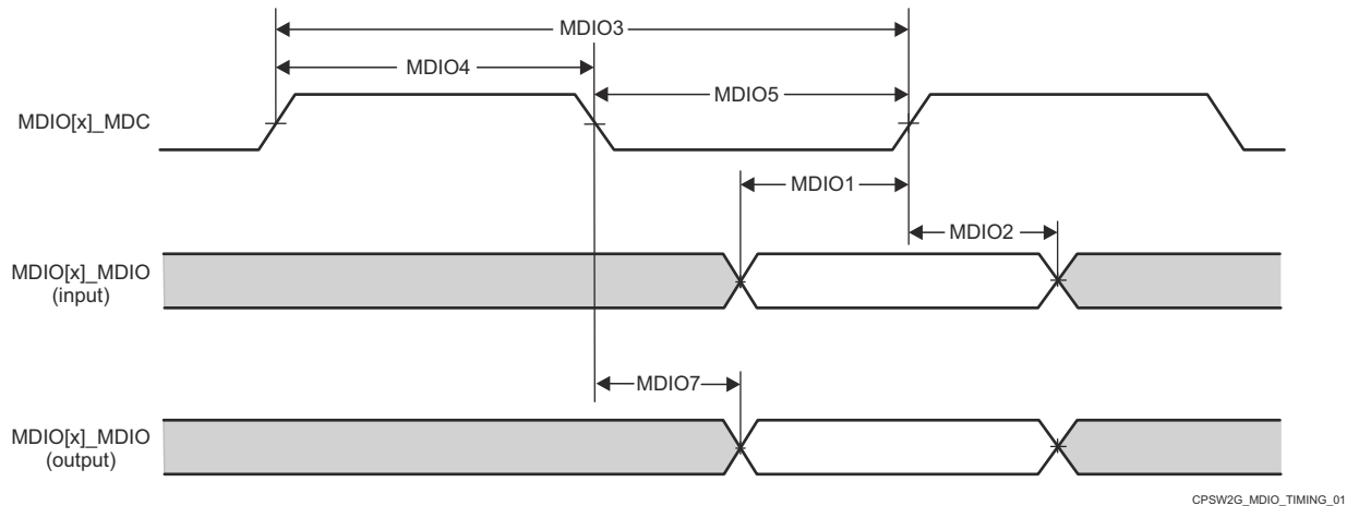
Figure 6-106. PRU_ICSSG MDIO Timing Requirements and Switching Characteristics
