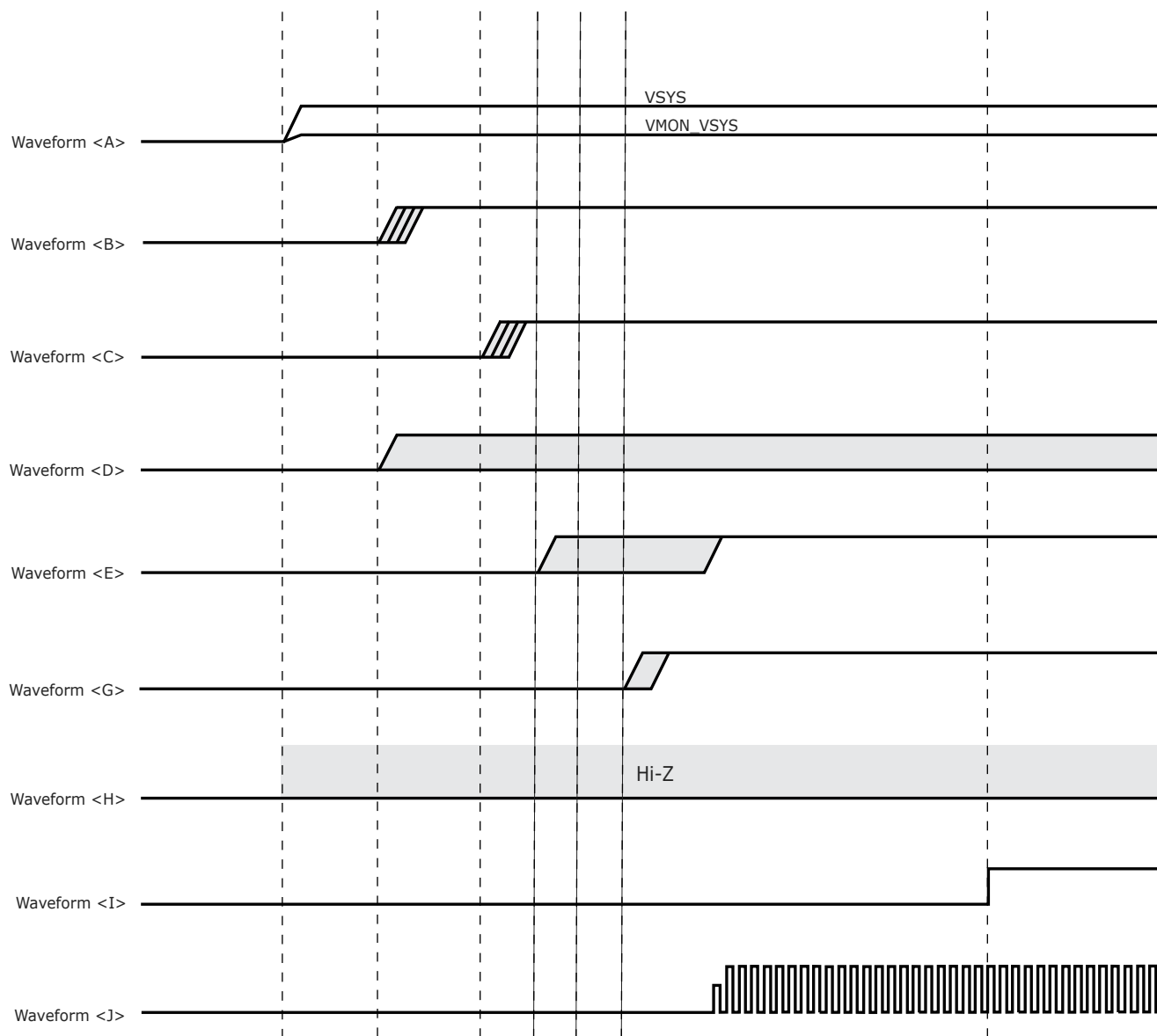
Figure 6-5. Power-Up Sequencing
