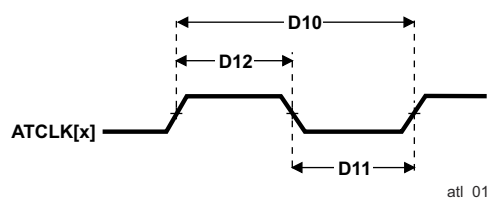
Figure 6-36. ATCLK[x] Timing
