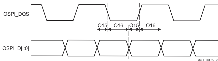
Figure 6-102. OSPI0/1 Timing Requirements – PHY Data Training, DDR with DQS
