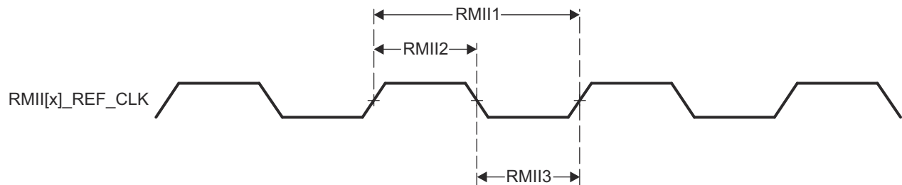
Figure 6-38. CPSW2G RMII[x]_REFCLK Timing Requirements – RMII Mode
