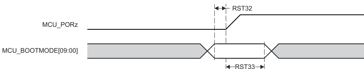
Figure 6-19. MCU_BOOTMODE Timing Requirements
