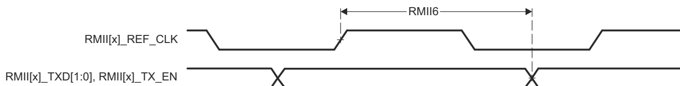
Figure 6-40. RMII[x]_TXD[1:0], and RMII[x]_TX_EN Switching Characteristics – RMII Mode
