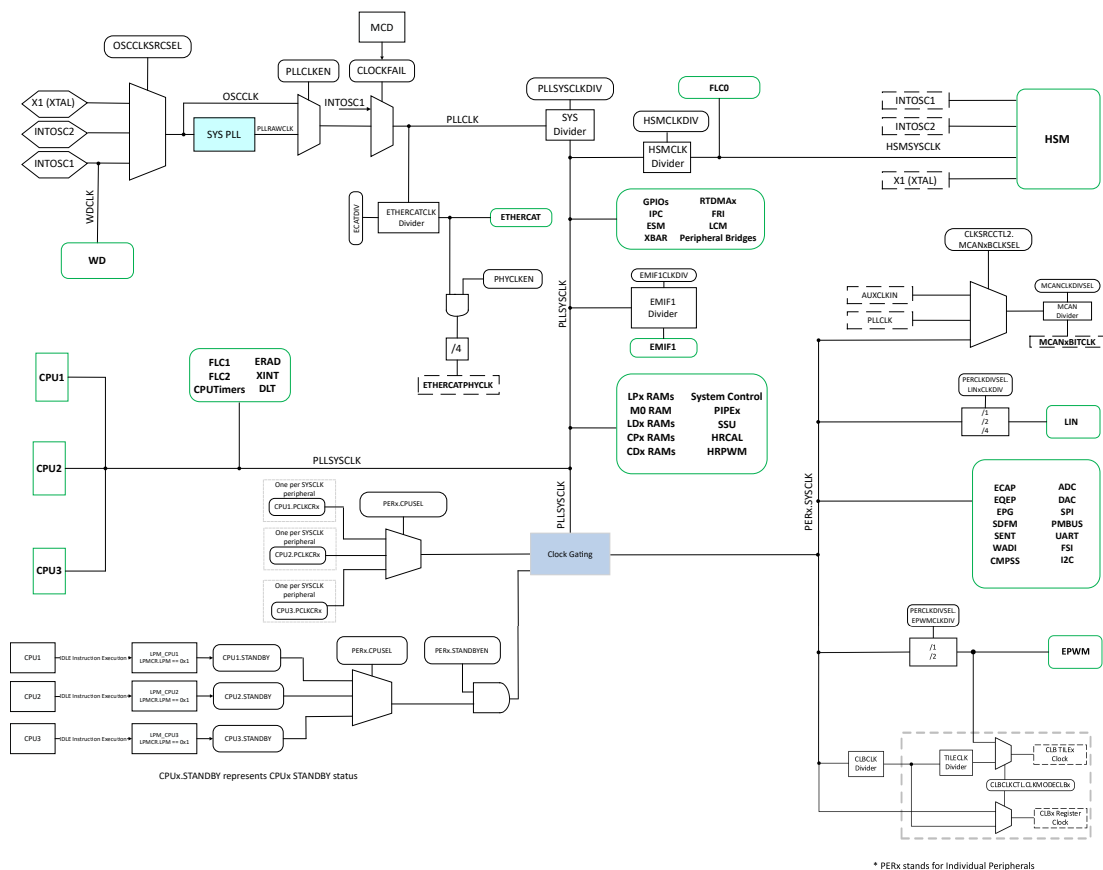
Figure 6-9. Clocking System
