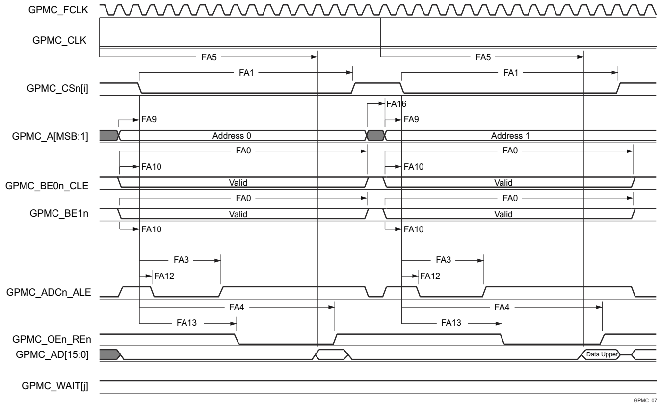
Figure 6-52. GPMC and NOR Flash — Asynchronous Read — Single Word
