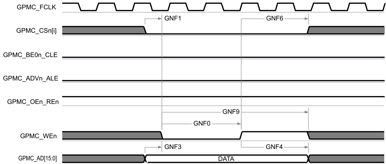
Figure 6-60. GPMC and NAND Flash — Data Read Cycle
