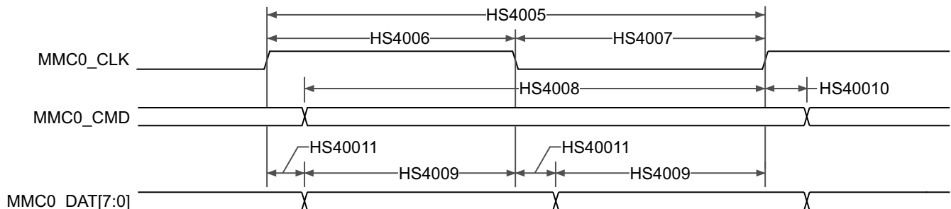
Figure 6-77. eMMC in – HS400 Mode – Transmitter Mode
