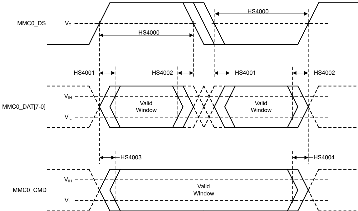
Figure 6-76. MMC0 – HS400 – Receive Mode
