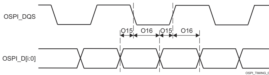
Figure 6-104. OSPI0 Timing Requirements – PHY DDR with External Board Loopback or DQS
