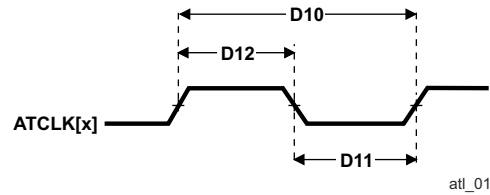
Figure 6-36. ATCLK[x] Timing
