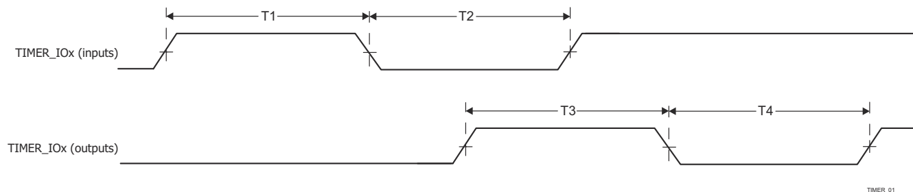
Figure 6-117. Timer Timing
