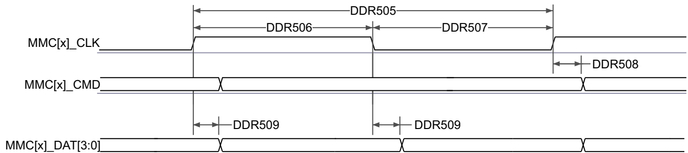
Figure 6-98. MMC1 – UHS-I DDR50 – Transmit Mode
