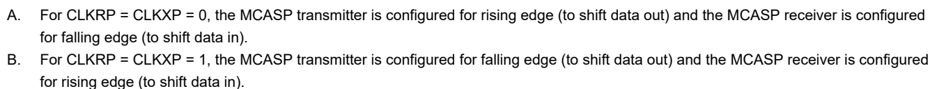
Figure 6-73. MCASP Input Timing
